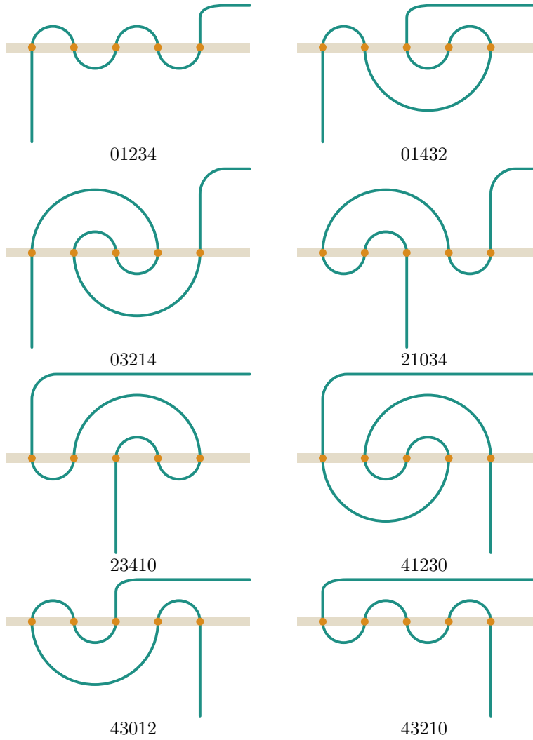
FIGURE 3. All eight open meanders with n = 5 crossings, each labelled with its crossing order (the bridges crossed, in river order, numbered from west to east). The river enters from the south; since n is odd, its last arc lies above the road and it leaves to the east above every other upper arc.
