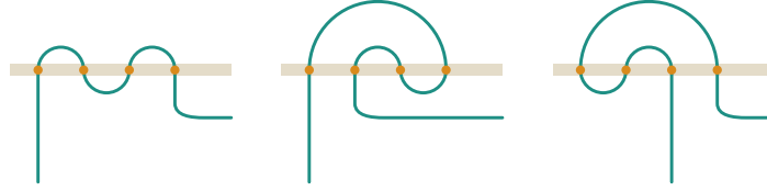
FIGURE 2. The three open meanders with n = 4 crossings. The river enters from the south and leaves to the east; bridges are numbered 0 to 3 from west to east. Their crossing orders are 0123, 0321 and 2103.
