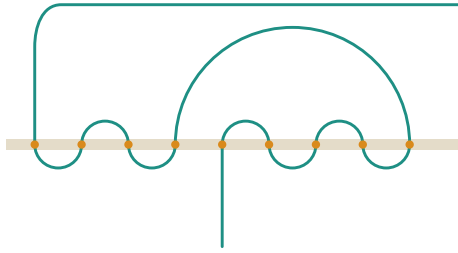
FIGURE 4. One of the 262 open meanders with n = 9 crossings; its crossing order is 456783210.
