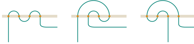
FIGURE 2. The three open meanders with n = 4 crossings. The river enters from the south and leaves to the east; bridges are numbered 0 to 3 from west to east. Their crossing orders are 0123, 0321 and 2103.
