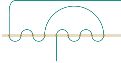
FIGURE 3. One of the 262 open meanders with n = 9 crossings.
