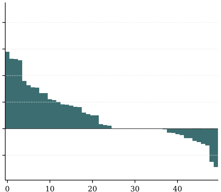
DL Hard
