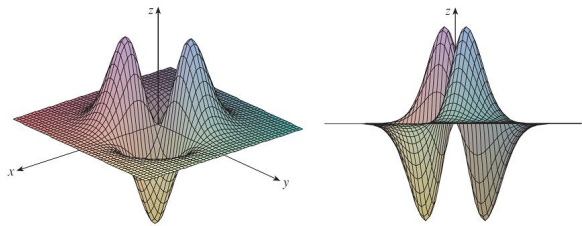
(b) Two views of f(x, y) = -xye^{-x^2-y^2}
