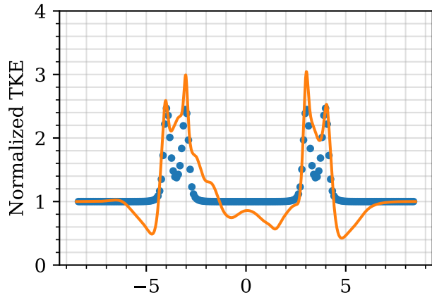
At 3D downstream first turbine
