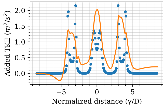
At 6D downstream first turbine
