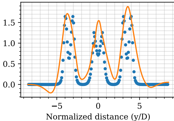
At 9D downstream first turbine
