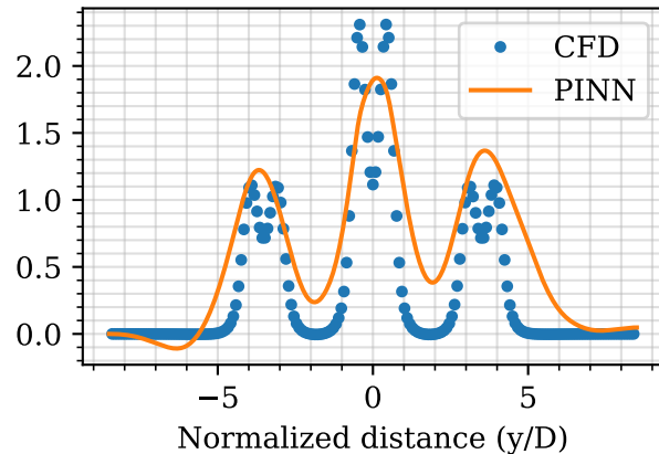
At 12D downstream first turbine
