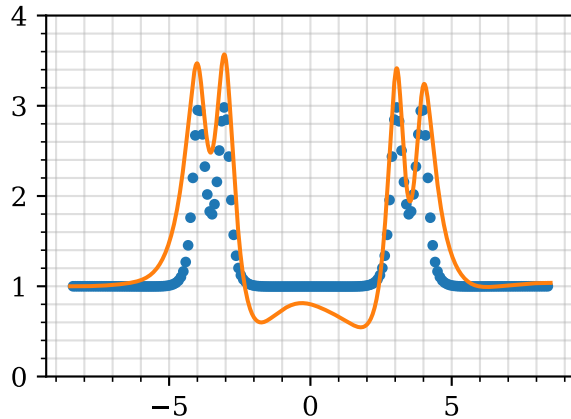
At 9D downstream first turbine
