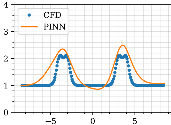
At 15D downstream first turbine
