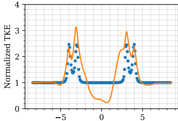
At 3D downstream first turbine
