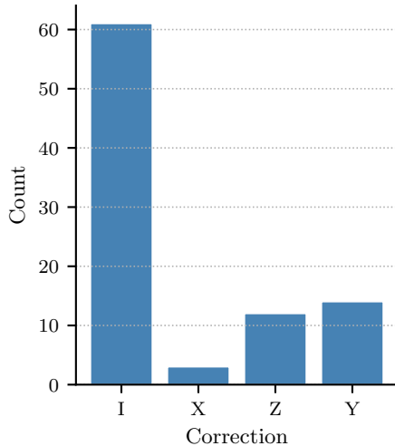
2-qubit errors (90)
