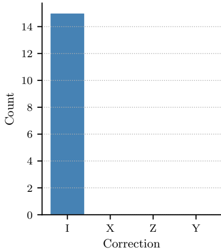
1-qubit errors (15)
