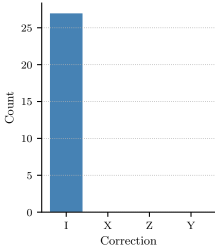
1-qubit errors (27)
