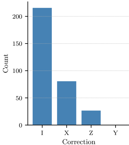
2-qubit errors (324)
