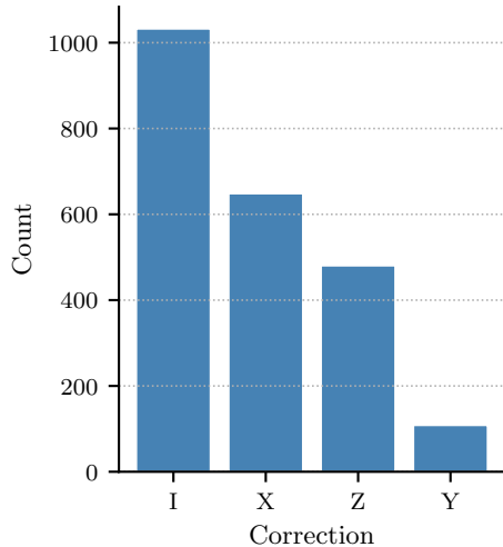
3-qubit errors (2268)
