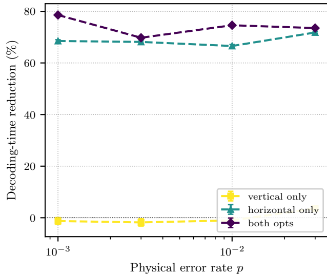
\chi_{\max} = 32 , ablation
