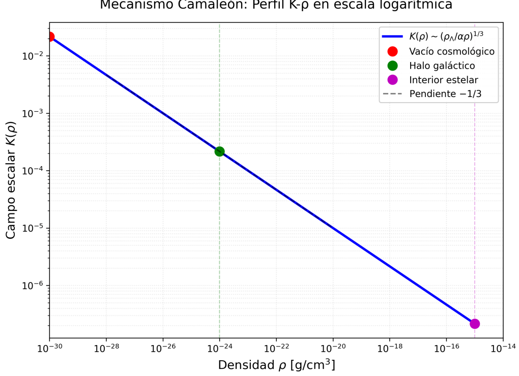
Figure 1: Chameleon profile \phi_{\min}(\rho) \sim (\rho_\Lambda/\alpha\rho)^{1/3} in log-log scale. The slope -1/3 confirms the power-law scaling across 15 decades in density. Three characteristic environments are marked: cosmological void ( \rho \sim 10^{-30} g cm -3 ), galactic halo ( \rho \sim 10^{-24} g cm -3 ), and stellar interior ( \rho \sim 10^{-15} g cm -3 ). The strong suppression at high density is the mechanism underlying Solar-System viability.
