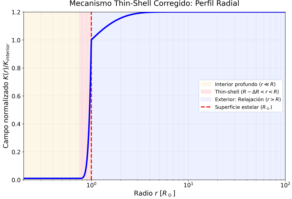
Figure 2: Radial profile of the normalized scalar field \phi(r)/\phi_{\text{int}} for a solar-type object. The strongly screened interior ( r \ll R_{\odot} ), the thin-shell transition region ( R_{\odot} - \Delta R < r < R_{\odot} ), and the exterior relaxation ( r > R_{\odot} ) are indicated. Only the thin-shell layer contributes to the exterior scalar force, enabling PPN compatibility.
