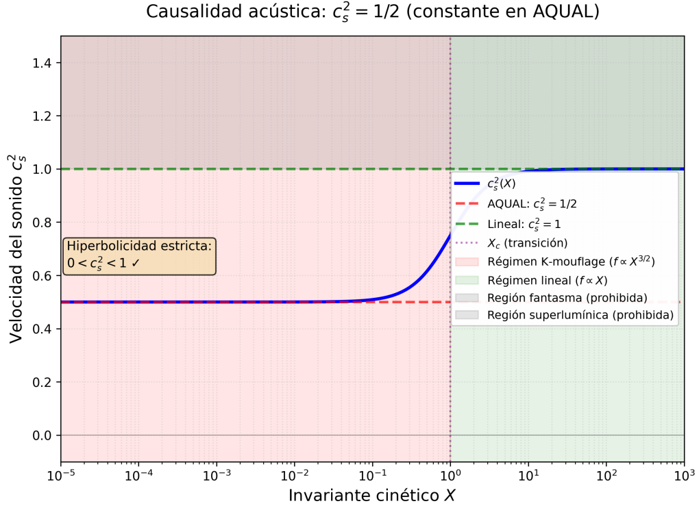
Figure 4: Effective sound speed c_s^2 as a function of the kinetic invariant X . In the AQUAL/k-mouflage regime ( X \ll X_c , relevant to galactic scales), c_s^2 = 1/2 exactly. In the Newtonian limit ( X \gg X_c , Solar-System scales), c_s^2 \rightarrow 1 . The permitted causal region 0 < c_s^2 < 1 ensures strict hyperbolicity and the absence of ghost instabilities throughout.
