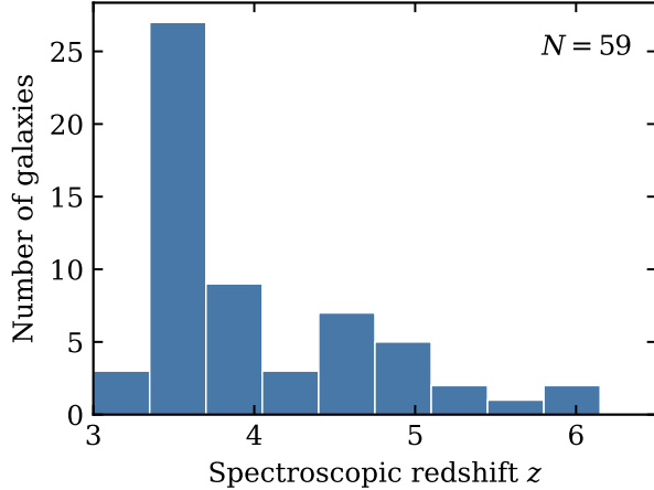
Fig. 1. Spectroscopic redshift distribution of the 59 JADES DR4 galaxies in the working sample. H\alpha is accessible with the NIRSpect medium-resolution gratings over the full z = 3 –6 range.
