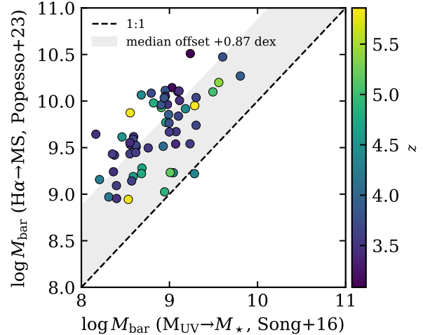
Fig. 5. Inter-method dispersion of baryonic masses. The \text{H}\alpha \rightarrow \text{SFR} \rightarrow \text{main-sequence} masses (used in the test) versus the M_{\text{UV}} \rightarrow M_{\star} masses for the same galaxies. The median offset is 0.87 dex (grey band), larger than the 0.45 dex mass reduction that would null the \Phi < 0 offset. The systematic floor of high- z masses exceeds the signal.
