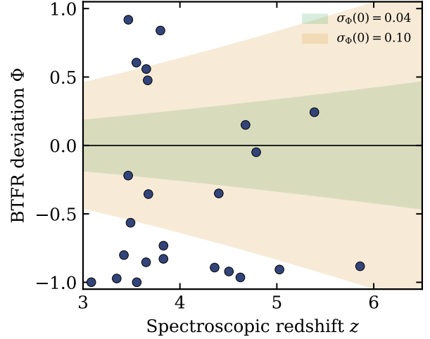
Fig. 4. BTFR deviation \Phi versus redshift for the Taylor-regime sample. Shaded bands show the \Lambda -EG prediction \pm \sigma_{\Phi}(0) H(z)/H_0 for \sigma_{\Phi}(0) = 0.04 dex (the §10.8 target) and 0.10 dex (measured). The data are offset to \Phi < 0 and scatter beyond the 0.04 dex band.
