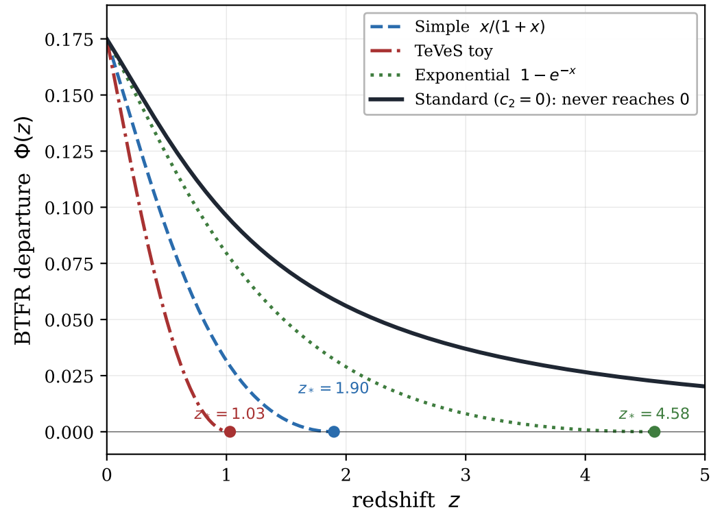
Excluded interpolants: c_2 \neq 0 \Rightarrow collapse at finite \lambda
