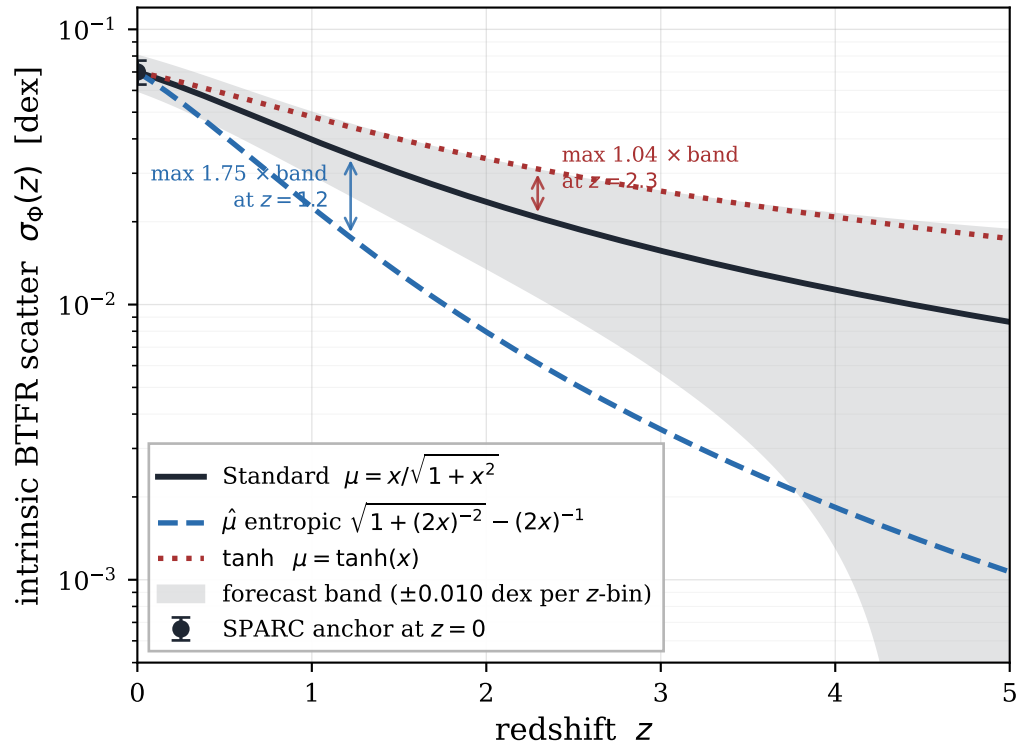
Surviving interpolants ( c_2 = 0 ): \sigma_\phi \propto (H/H_0)^{\beta'_{(0)}}
