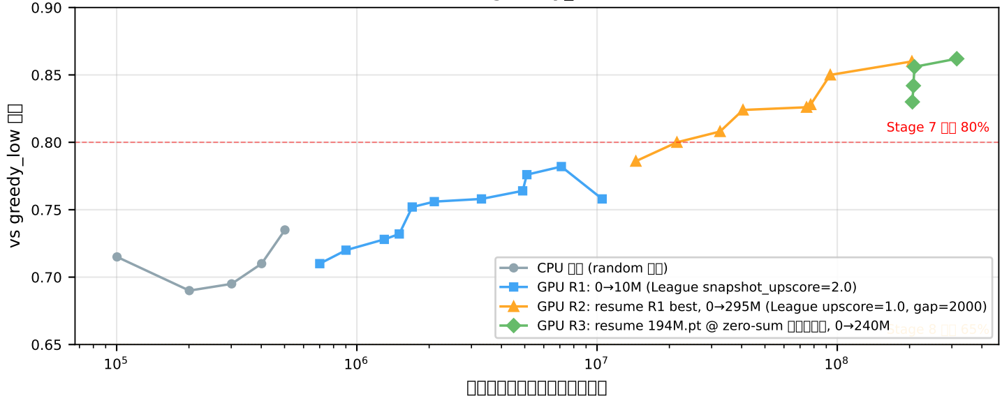
Best vs greedy_low
