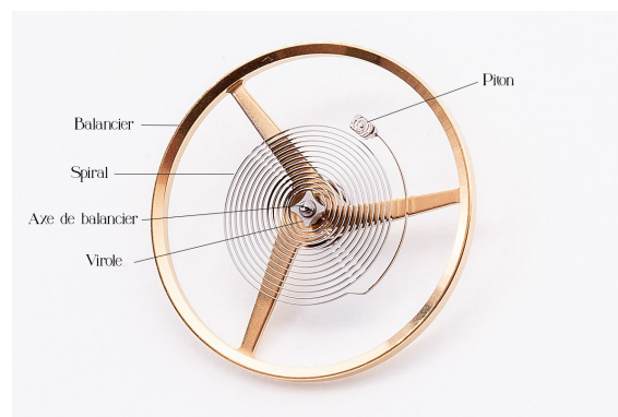
Figure 2.6 – Balancier-spiral [6]
