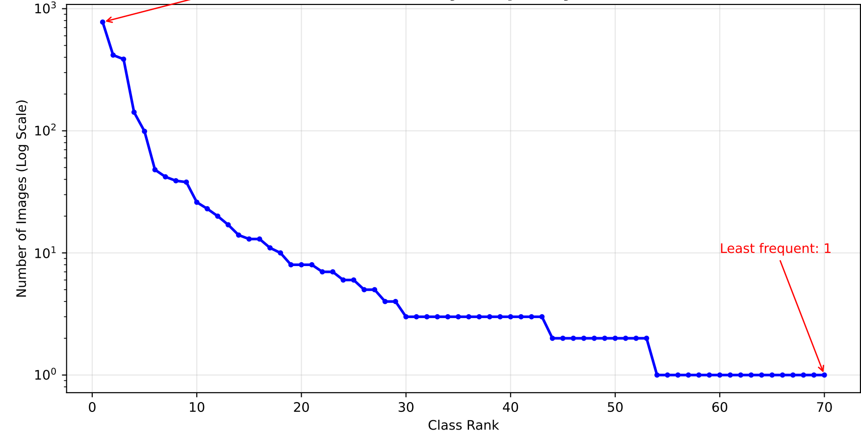
Class Imbalance Pattern (Ranked by Frequency)
