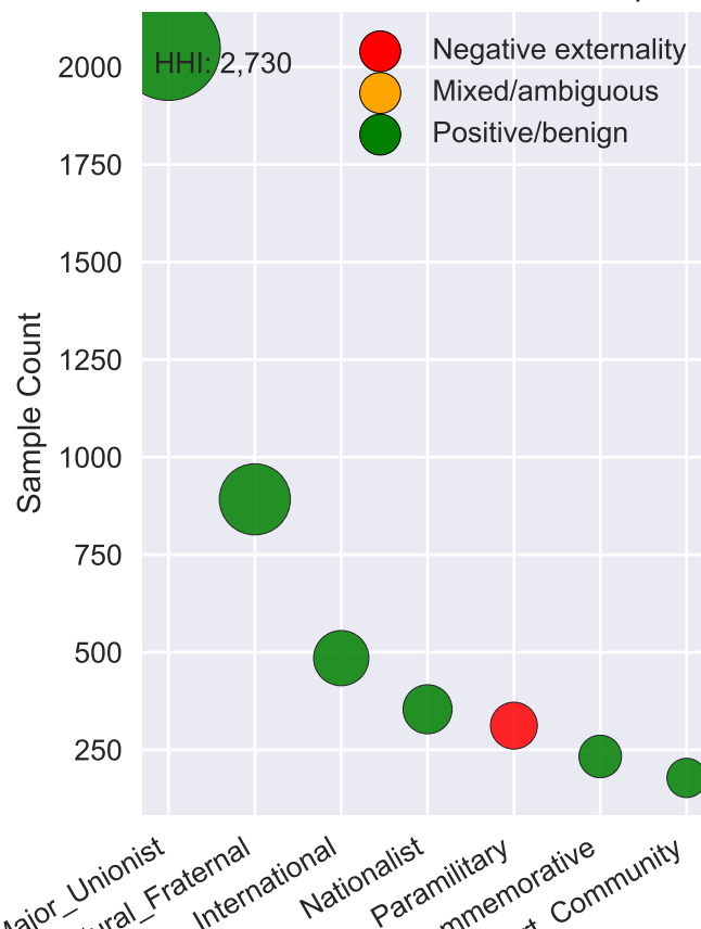
Economic Externalities vs Samples
