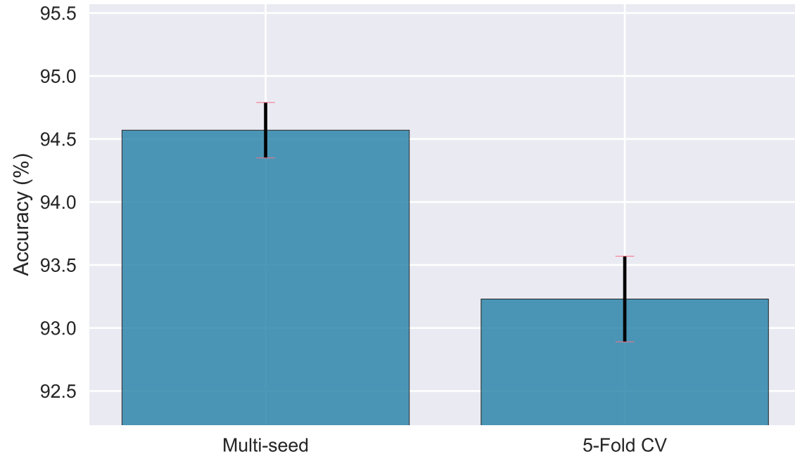
Statistical Validation
