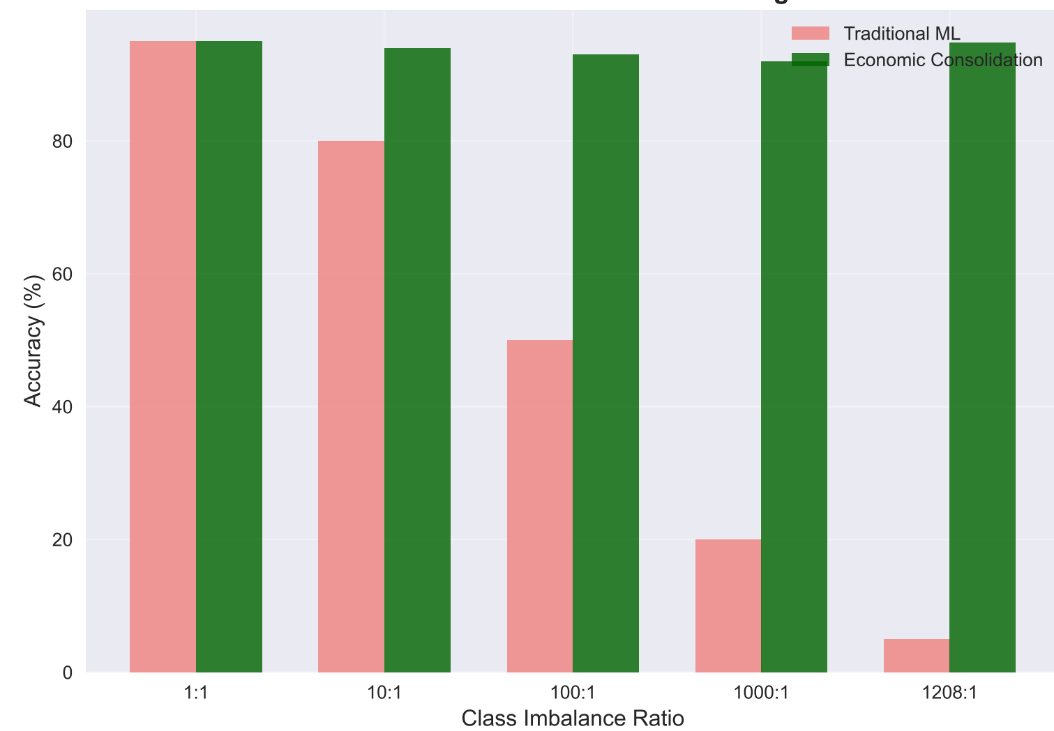
Extreme Class Imbalance Handling
