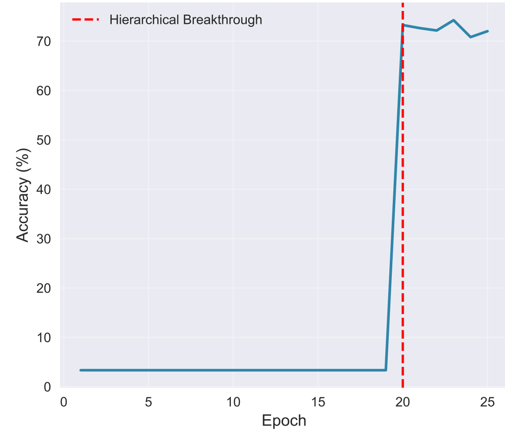
Training Dynamics
