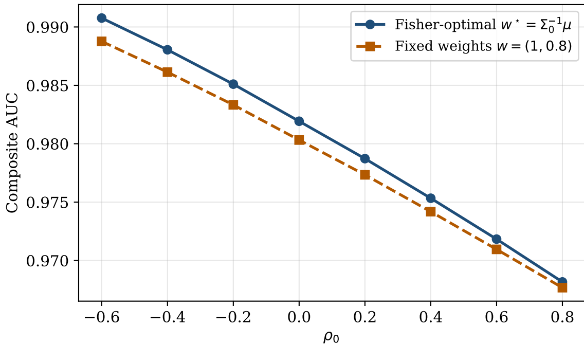
Efficiency loss from weight misspecification ( \sigma_\varepsilon = 0.25 )
