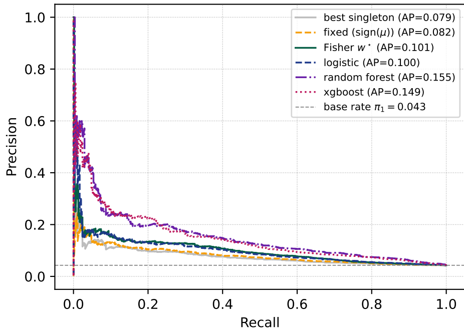
Precision-Recall
