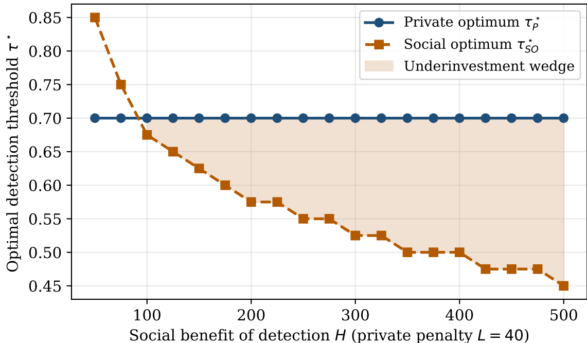
Private vs social thresholds (lower \tau = more intense monitoring)
