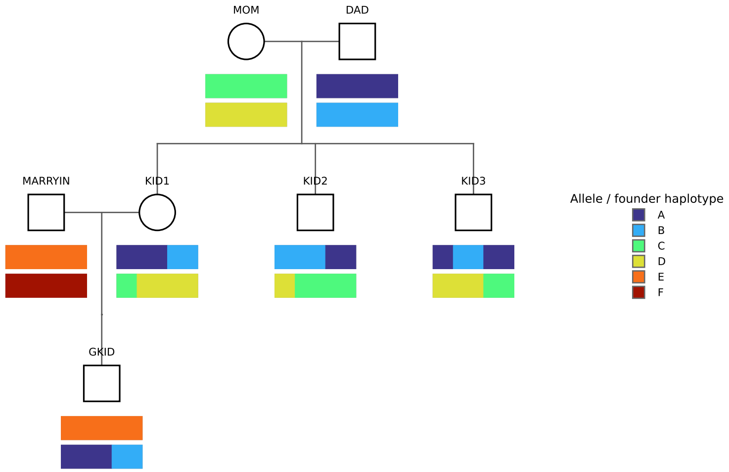
Pedigree haplotype painting — chr1 (1.00–9.00 Mb, apex trios relabelled A,B,C,D)
