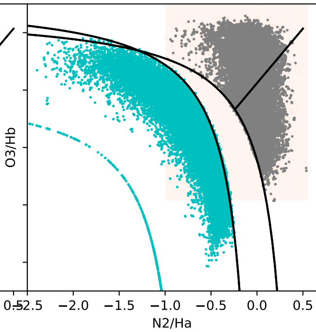
Generated Data w/0.01 dex scatter
