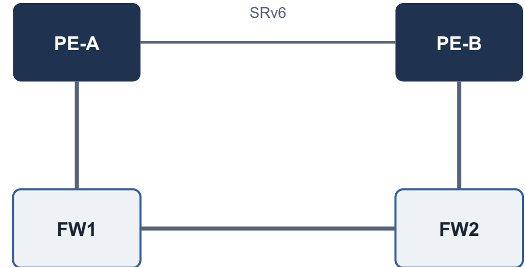
Case 2: two firewalls in a square
