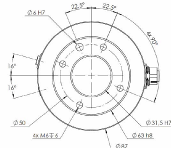
TCP Flange Hole Pattern for LARA 3/5/8/10
