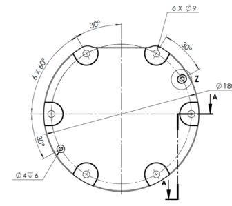
Robot Base Hole Pattern for LARA 8/10
