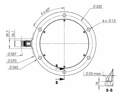
Robot Base Hole Pattern for LARA 15
