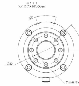
TCP Flange Hole Pattern for LARA 20
