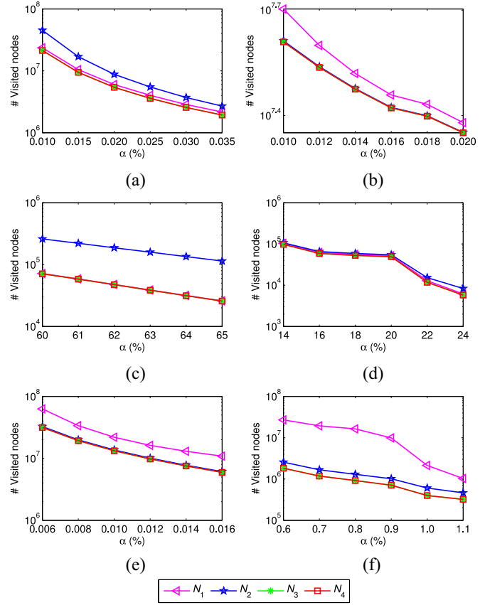
Fig. 6. Number of visited nodes under varied \alpha with a fixed \beta . (a) BMSPOS2 ( \beta:0.3 ). (b) retail ( \beta:0.3 ). (c) chess ( \beta:0.3 ). (d) mushroom ( \beta:0.3 ). (e) T10I4D100K ( \beta:0.3 ). (f) T40I10D100K ( \beta:0.3 ).
