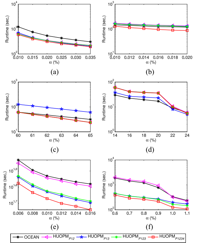
Fig. 4. Runtime under varied \alpha with a fixed \beta . (a) BMSP0S2 ( \beta:0.3 ). (b) retail ( \beta:0.3 ). (c) chess ( \beta:0.3 ). (d) mushroom ( \beta:0.3 ). (e) T10I4D100K ( \beta:0.3 ). (f) T40I10D100K ( \beta:0.3 ).
