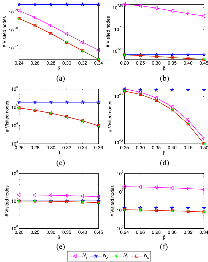
Fig. 7. Number of visited nodes under varied \beta with a fixed \alpha . (a) BMSPOS2 ( \alpha:0.02\% ). (b) retail ( \alpha:0.014\% ). (c) chess ( \alpha:62\% ). (d) mushroom ( \alpha:18\% ). (e) T10I4D100K ( \alpha:0.012\% ). (f) T40I10D100K ( \alpha:0.8\% ).
