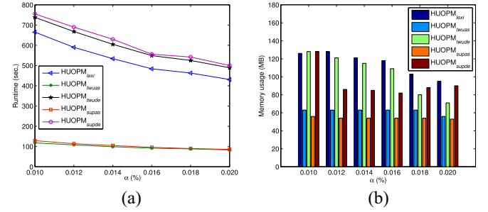
Fig. 8. Effect of processing order of items (five types of processing orders: HUOPM_{lexi} , HUOPM_{twuas} , HUOPM_{twde} , HUOPM_{supas} , and HUOPM_{supde} ). (a) retail ( \beta:0.3 ). (b) retail ( \beta:0.3 ).
