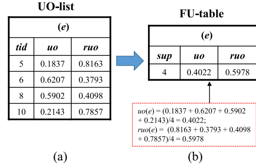
Fig. 2. UO-list and FU-table of item (e).
