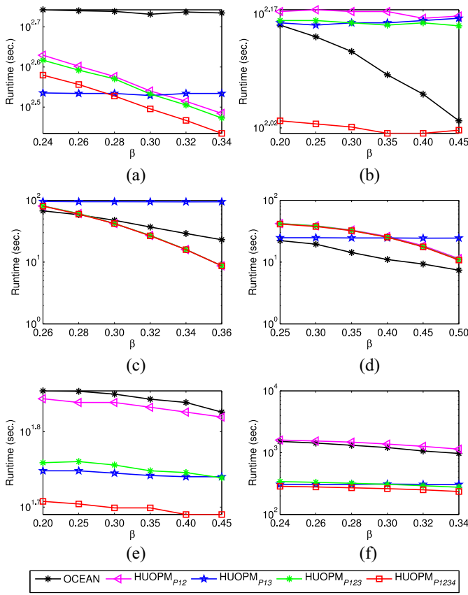
Fig. 5. Runtime under varied \beta with a fixed \alpha . (a) BMSPOS2 ( \alpha:0.02\% ). (b) retail ( \alpha:0.014\% ). (c) chess ( \alpha:62\% ). (d) mushroom ( \alpha:18\% ). (e) T10I4D100K ( \alpha:0.012\% ). (f) T40I10D100K ( \alpha:0.8\% ).
