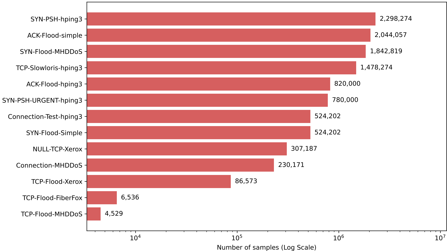
Use case 2: TCP-based DDoS Attack - IoT-IDS-Zwave-2025: Class Distribution
