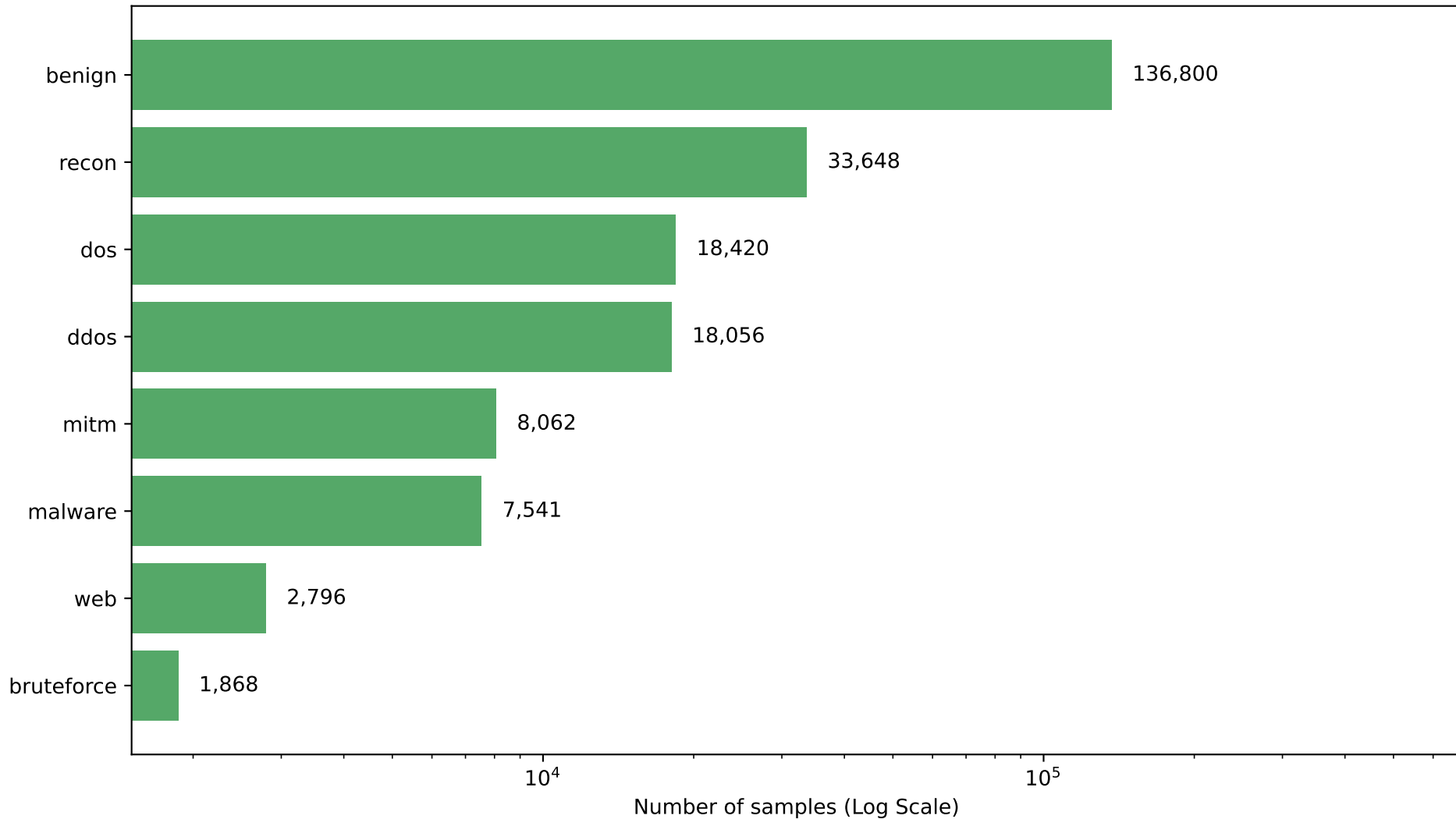
Use case 3: CIC IIOT 2025: Class Distribution
