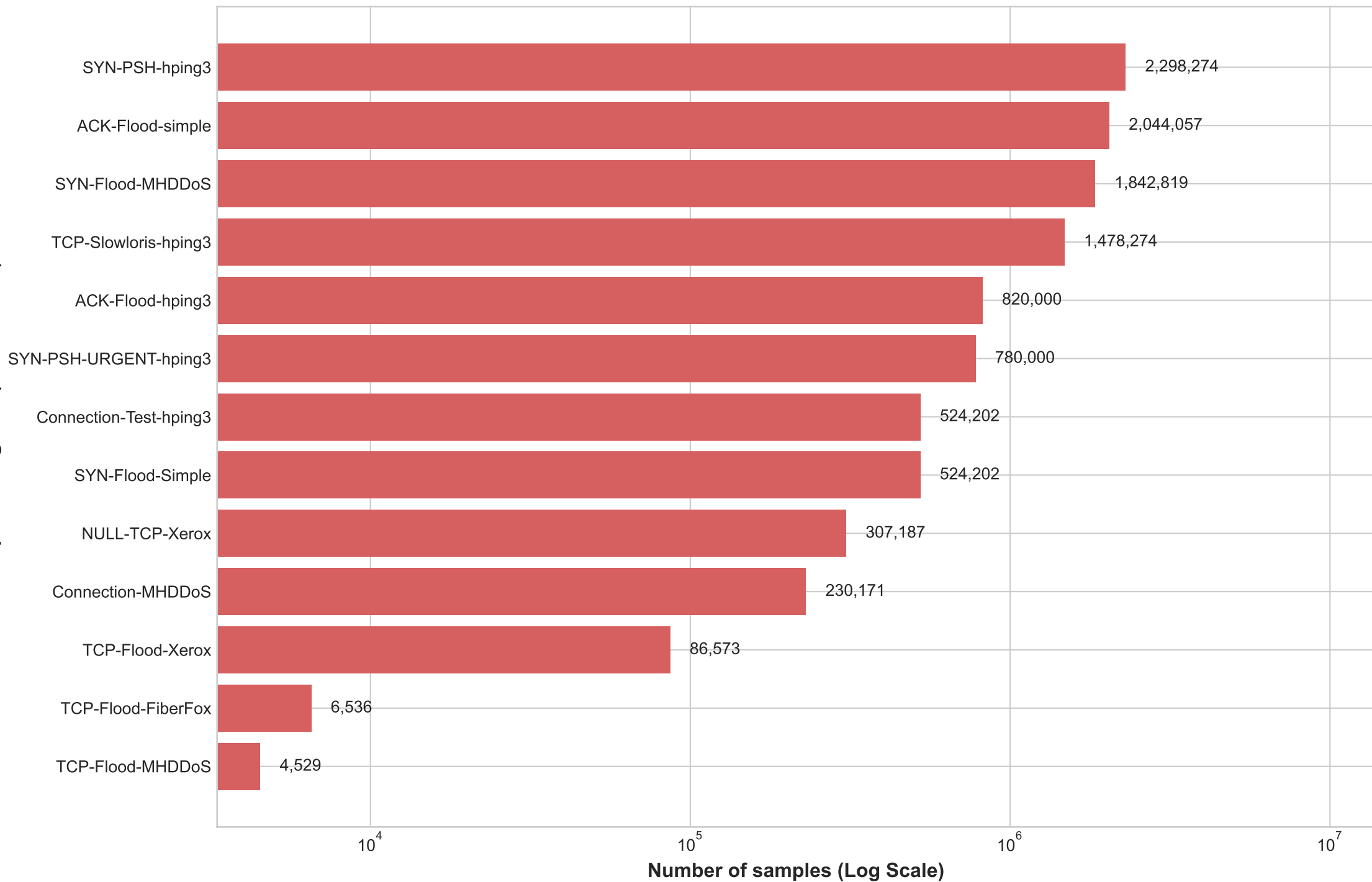
Use case 2: Application-based DDoS Attack - IoT-IDS-Zwave-2025: Class Distribution
