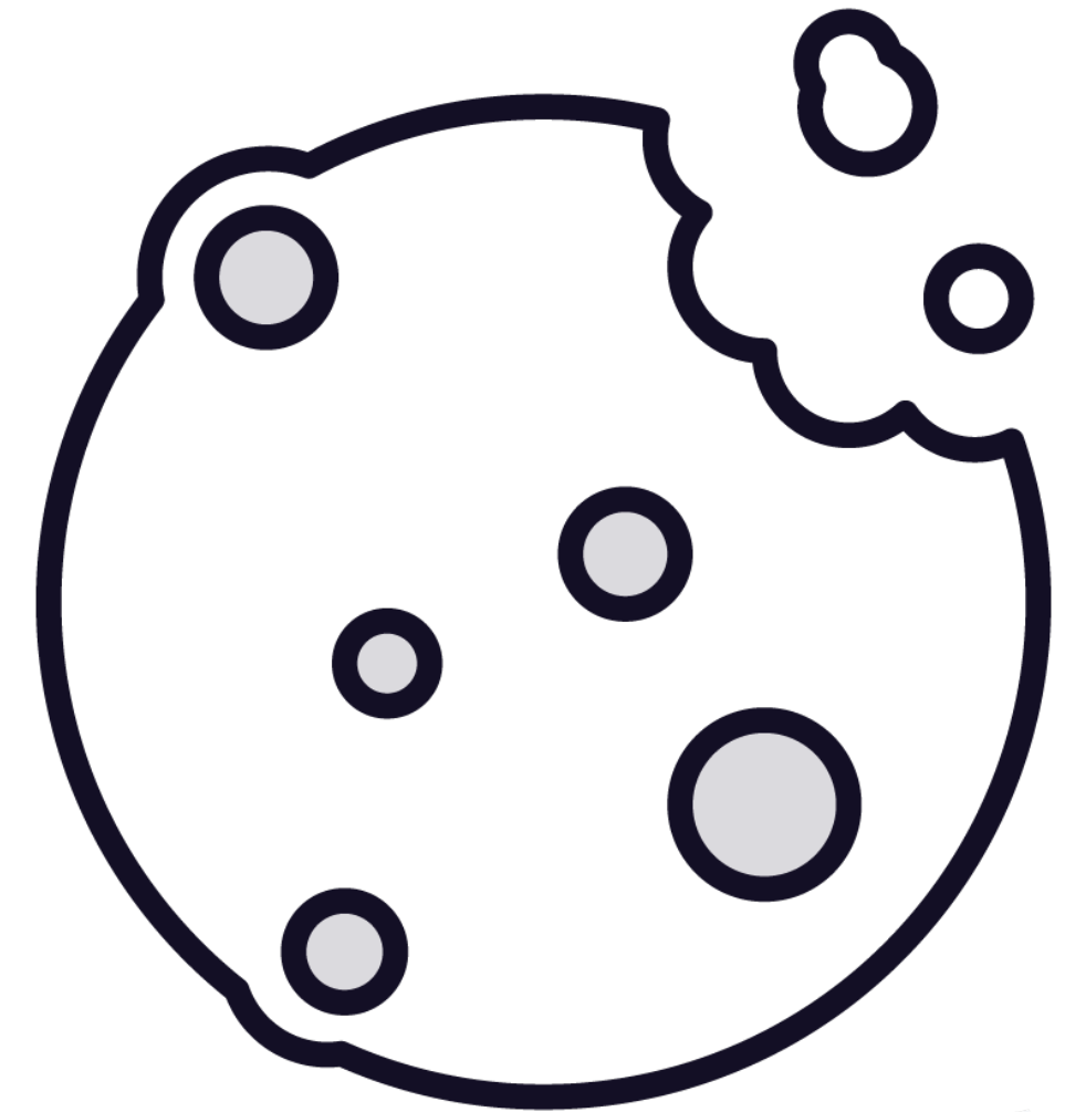
HTTP Cookies
