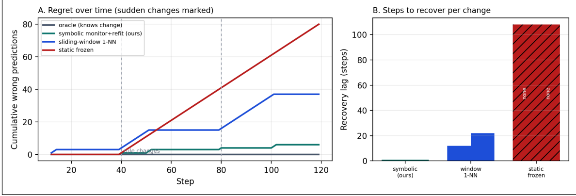
Figure 17: Adapting to sudden unannounced rule changes (E41). A reservoir’s hidden regime jumps at the marked steps; predictions run through the perception boundary. A: cumulative wrong predictions—the symbolic monitor (ours) stays nearly flat, the sliding-window learner steps up and slowly recovers, the static-frozen model climbs without bound, the oracle is flat at zero. B: recovery lag per change—1/1 steps for the symbolic monitor (to exact) versus 12/22 for the window; the frozen model never recovers.
