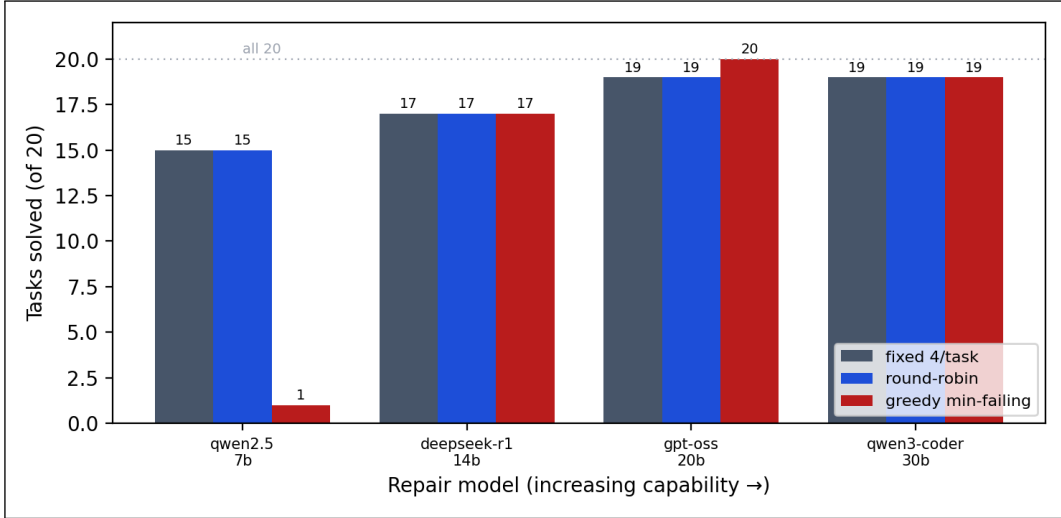
Figure 14: The sprint allocation across a capability ladder (E35). Tasks solved on OpenWorld-SWE-bench under the three allocation conditions, by repair model (increasing capability left to right; budget 80). The fixed-protocol ceiling rises with capability; the greedy tarpit (a lone solved task at 7B) defangs with scale, clearing all 20 at gpt-oss:20b.
