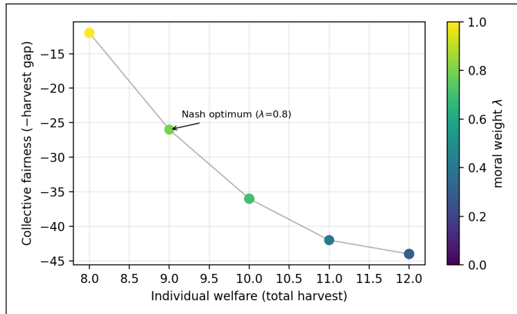
Figure 7: Tunable morality (E8). The welfare–fairness frontier traced by sweeping the moral dial \lambda on the commons world. Every point is Pareto-optimal; the Nash bargaining optimum is interior. Values are declared, weighted artifacts—moving along this frontier requires no retraining.
