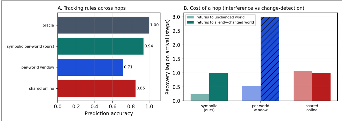
Figure 18: Agents traversing connected worlds with changing rules (E42). Two worlds joined by a toll route, each non-stationary, each with its own perception boundary; an agent hops between them. A: prediction accuracy tracking the current world’s rule across hops. B: recovery lag on arrival, split by whether the world’s rule changed while the agent was away. The shared-belief learner pays an interference cost even returning to an unchanged world; the per-world symbolic monitor returns nearly free and re-identifies away-changes in a step; the per-world window does not reliably recover from away-changes within a visit (hatched = no recovery).
