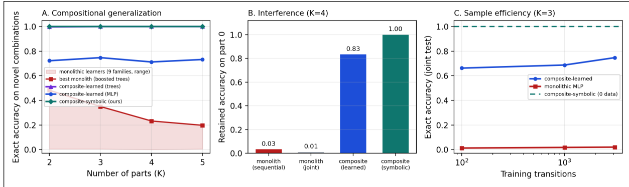
Figure 15: Composition vs. monolithic learners (E36) on a factored K -sector world, capacity-fair. A: exact accuracy on novel sector combinations—the whole monolithic family (shaded range over 9 learners; best, boosted trees, shown) collapses as K grows, while both composite learners and the symbolic composite stay flat near or at 1.0. B: accuracy retained on the first part after training through all K —the monolith suffers catastrophic interference, the composite does not. C: accuracy vs. training transitions—the composite learns from far less data, the symbolic composite from none.
