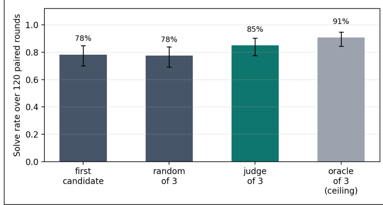
Figure 6: Controlled judge-selection comparison (E13+E17, pooled). Four selection strategies over the same three 1.5B candidate patches per round, 120 paired rounds; whiskers are 95% Wilson intervals. Random-of-3 isolates the diversity effect; the judge’s margin over it estimates the value of judgment (McNemar p = 0.078 , marginal).
