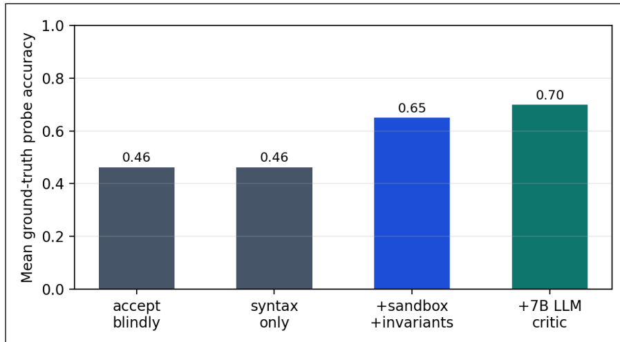
Figure 5: Verifier ablation (E3). Semantic correctness of accepted sprint-world dynamics under four acceptance regimes; eight paired high-temperature 3B generations per condition, graded against ground truth on a branch-covering probe suite.
