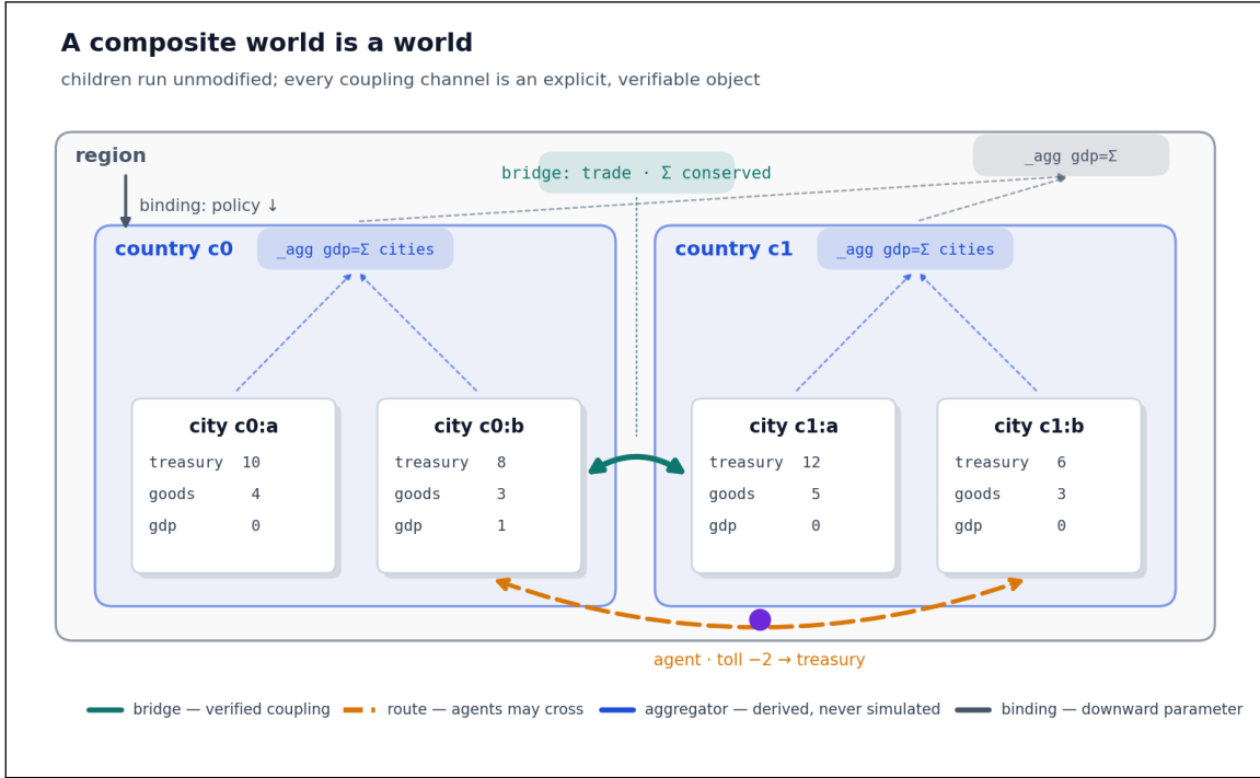
Figure 9: Anatomy of a composite world (the E31 system, real state values). Two country worlds, each containing two unmodified city worlds, compose into a region. The four coupling channels are explicit objects: a verified bridge carries trade under a conservation invariant; a dashed route lets an agent cross (paying a toll into the destination treasury); dashed upward arrows are aggregators —parent summaries derived from leaves, never independently simulated; the solid downward arrow is a binding injecting a parent parameter into a child.
