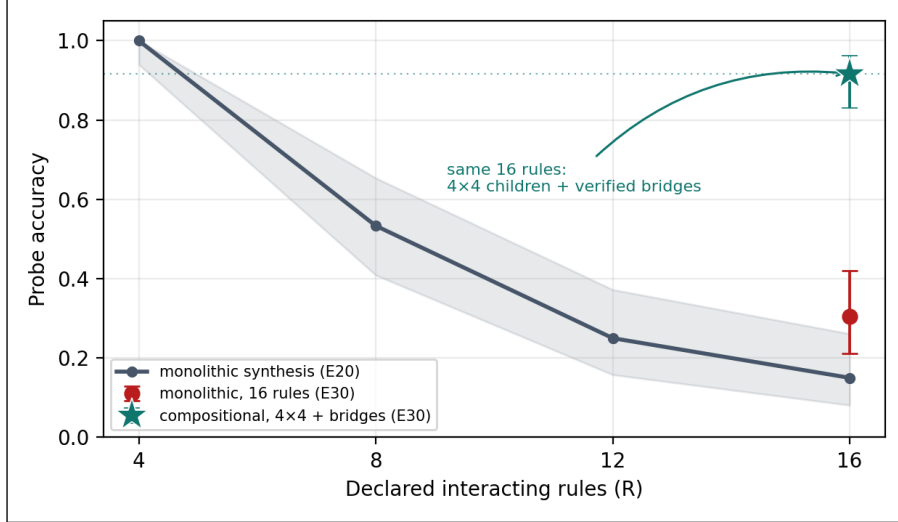
Figure 10: Composition defeats the cliff. The E20 curve (grey, with pooled 95% CI band): monolithic 7B synthesis accuracy falls as declared interacting rules grow. At R=16 , E30’s monolithic condition (red) lands on the fallen curve, while the same sixteen rules synthesized as four 4-rule children plus verified bridges (teal star) return to near- R=4 accuracy.
