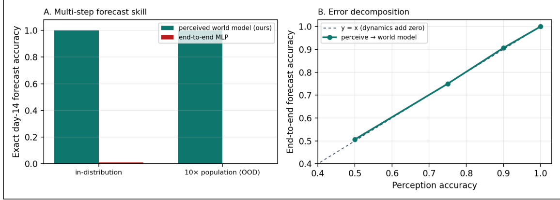
Figure 17: Perceive-then-forecast (E40). Multimodal day-0 inputs are perceived into the symbolic state of an SIR epidemic, then rolled forward 14 days by the verified world model. A: exact day-14 forecast accuracy—the perceived world model is exact in and out of distribution; the end-to-end MLP fails and collapses at 10 \times scale. B: end-to-end forecast accuracy equals perception accuracy (the dynamics add zero error), so the system degrades only as fast as its perception does.
