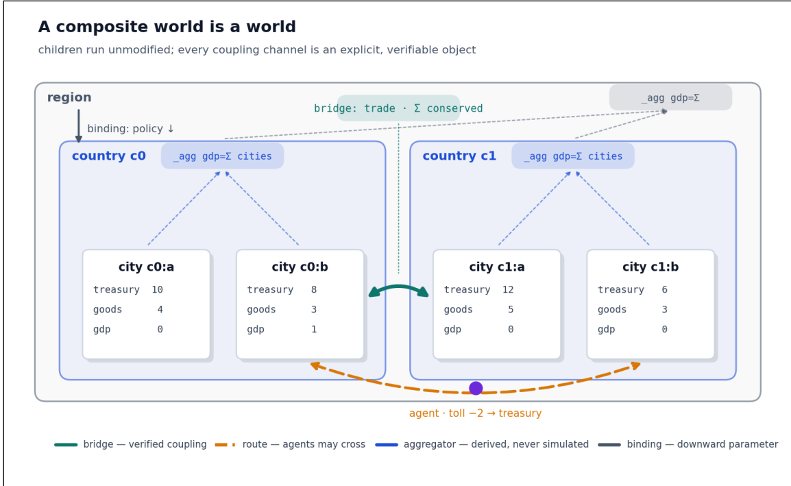
Figure 10: Anatomy of a composite world (the E31 system, real state values). Two country worlds, each containing two unmodified city worlds, compose into a region. The four coupling channels are explicit objects: a verified bridge carries trade under a conservation invariant; a dashed route lets an agent cross (paying a toll into the destination treasury); dashed upward arrows are aggregators —parent summaries derived from leaves, never independently simulated; the solid downward arrow is a binding injecting a parent parameter into a child.
