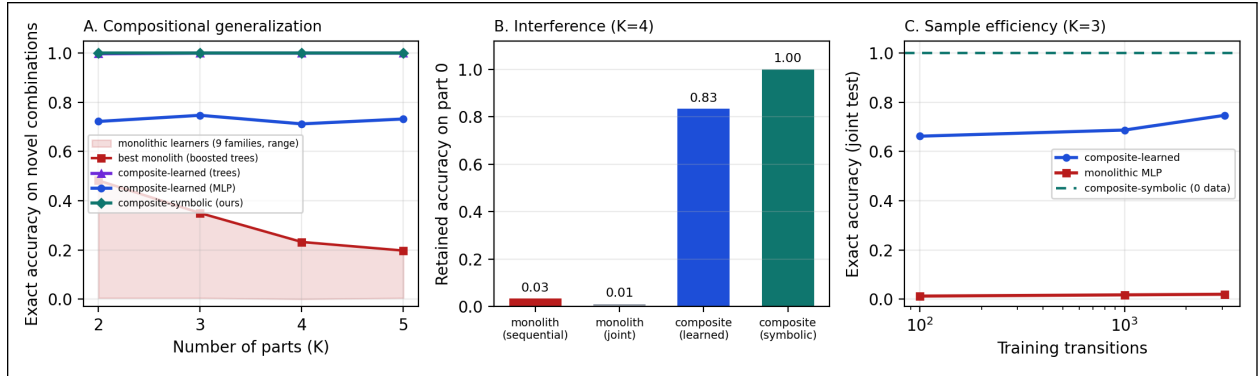
Figure 16: Composition vs. monolithic learners (E36) on a factored K -sector world, capacity-fair. A: exact accuracy on novel sector combinations—the whole monolithic family (shaded range over 9 learners; best, boosted trees, shown) collapses as K grows, while both composite learners and the symbolic composite stay flat near or at 1.0. B: accuracy retained on the first part after training through all K —the monolith suffers catastrophic interference, the composite does not. C: accuracy vs. training transitions—the composite learns from far less data, the symbolic composite from none.
