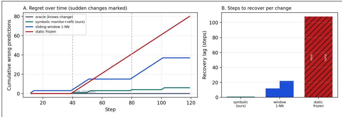
Figure 18: Adapting to sudden unannounced rule changes (E41). A reservoir’s hidden regime jumps at the marked steps; predictions run through the perception boundary. A: cumulative wrong predictions—the symbolic monitor (ours) stays nearly flat, the sliding-window learner steps up and slowly recovers, the static-frozen model climbs without bound, the oracle is flat at zero. B: recovery lag per change—1/1 steps for the symbolic monitor (to exact) versus 12/22 for the window; the frozen model never recovers.
