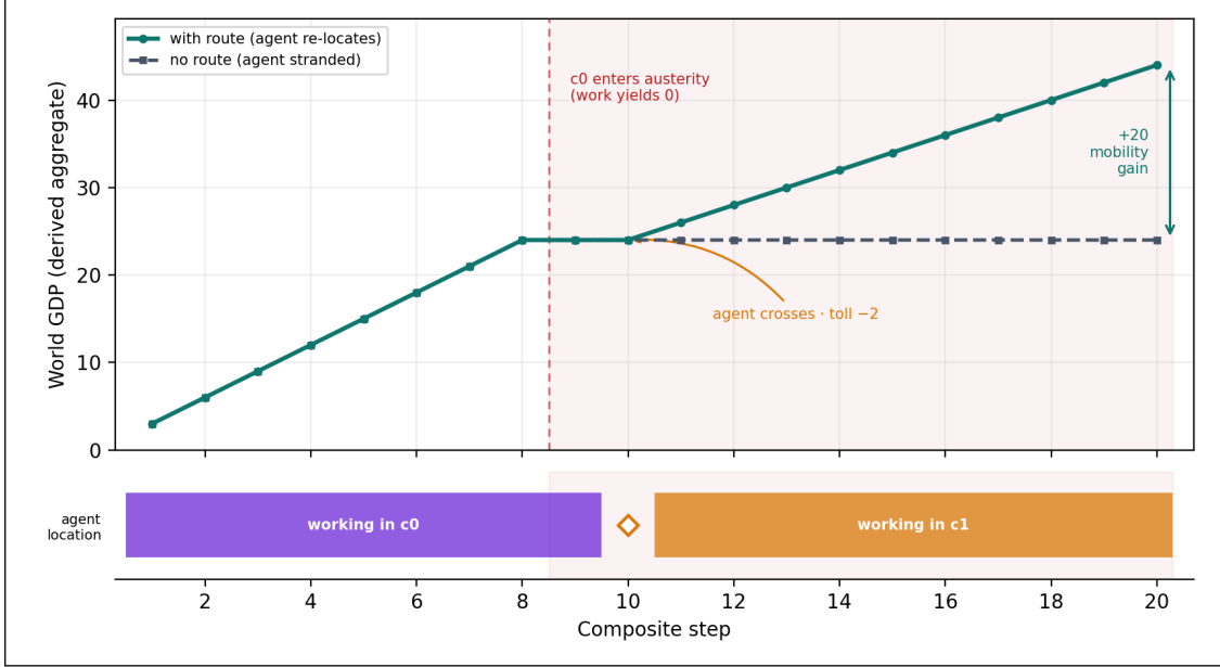
Figure 13: When the rules change, agents move (E33, deterministic). Top: world GDP with and without the route; the shaded band is the home economy’s austerity regime, entered at step 9. The agent observes the collapsed rate, crosses at step 10 (toll -2 ), and growth resumes in the destination economy; the stranded counterfactual flatlines, leaving a +20 mobility gain. Bottom: the agent’s location lane on the same time axis.
