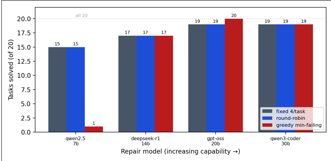
Figure 15: The sprint allocation across a capability ladder (E35). Tasks solved on OpenWorld-SWE-bench under the three allocation conditions, by repair model (increasing capability left to right; budget 80). The fixed-protocol ceiling rises with capability; the greedy tarpit (a lone solved task at 7B) defangs with scale, clearing all 20 at gpt-oss:20b.
