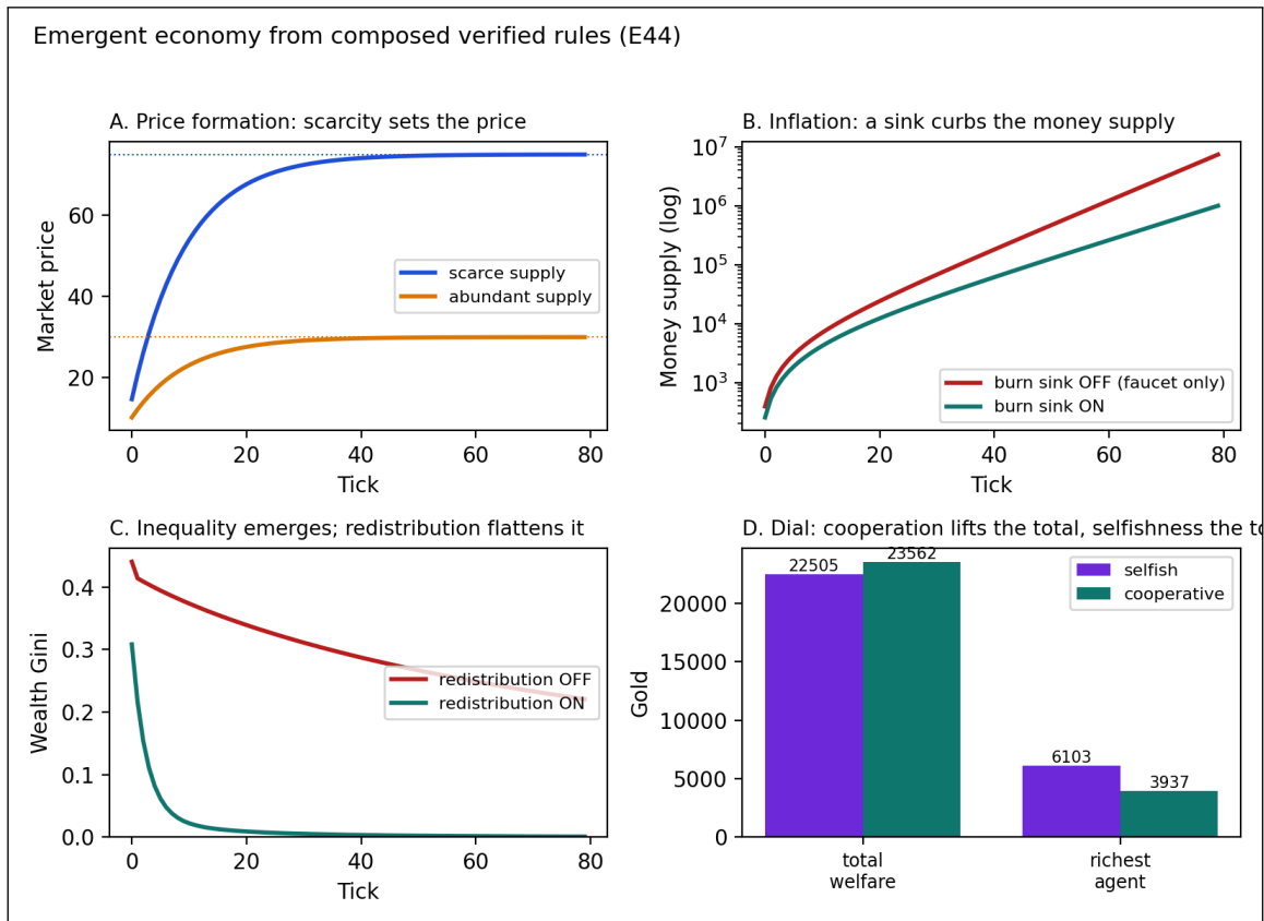
Figure 20: Emergent economy from composed verified rules (E44). Four macro phenomena, each isolated by toggling one verified rule. A: price converges to a supply-set level (scarcer supply \Rightarrow higher price). B: money supply (log) inflates with the burn sink off; the sink curbs it. C: the wealth Gini rises under selfish accumulation; redistribution flattens it. D: cooperation raises total welfare while selfishness produces the single richest agent. Nothing in the rules targets these quantities; they emerge and are causally attributed by separable toggles.
