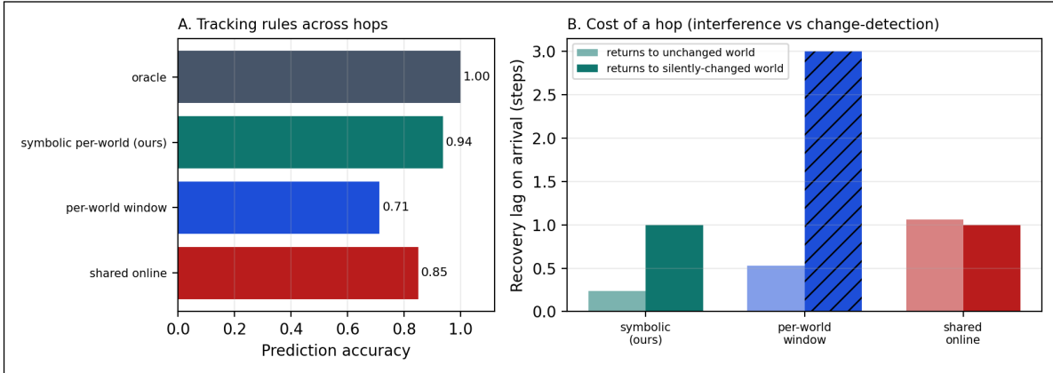
Figure 19: Agents traversing connected worlds with changing rules (E42). Two worlds joined by a toll route, each non-stationary, each with its own perception boundary; an agent hops between them. A: prediction accuracy tracking the current world’s rule across hops. B: recovery lag on arrival, split by whether the world’s rule changed while the agent was away. The shared-belief learner pays an interference cost even returning to an unchanged world; the per-world symbolic monitor returns nearly free and re-identifies away-changes in a step; the per-world window does not reliably recover from away-changes within a visit (hatched = no recovery).
