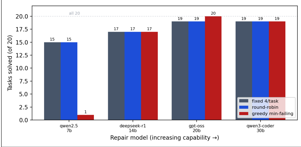
Figure 20: The sprint allocation across a capability ladder (E35). Tasks solved on OpenWorld-SWE-bench under the three allocation conditions, by repair model (increasing capability left to right; budget 80). The fixed-protocol ceiling rises with capability; the greedy tarpit (a lone solved task at 7B) defangs with scale, clearing all 20 at gpt-oss:20b.
