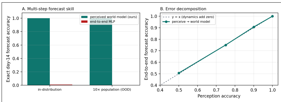
Figure 19: Perceive-then-forecast (E40). Multimodal day-0 inputs are perceived into the symbolic state of an SIR epidemic, then rolled forward 14 days by the verified world model. A: exact day-14 forecast accuracy—the perceived world model is exact in and out of distribution; the end-to-end MLP fails and collapses at 10\times scale. B: end-to-end forecast accuracy equals perception accuracy (the dynamics add zero error), so the system degrades only as fast as its perception does.
