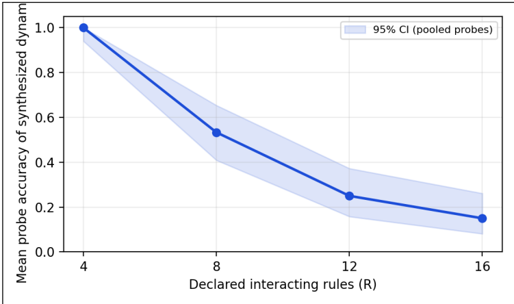
Figure 11: The complexity cliff (E20). Probe accuracy of 7B-synthesized dynamics versus the number of declared interacting rules; three syntheses per point, shaded band is the 95% CI over pooled probes. Monolithic synthesis is reliable at R=4 and unreliable past R \approx 8 .
