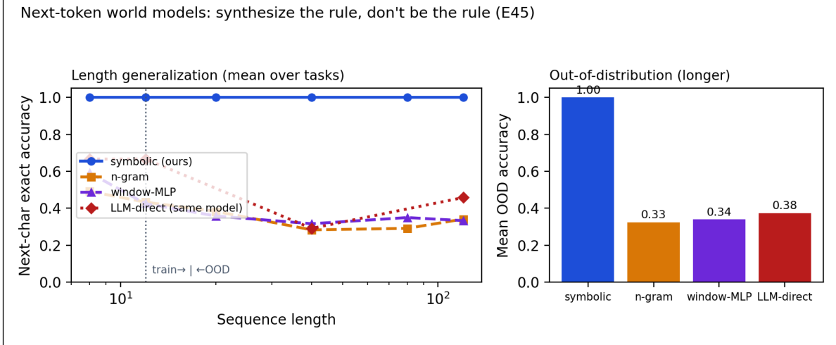
Figure 7: Next-token world models (E45). Left: next-character accuracy vs. sequence length (mean over tasks). The induced symbolic program stays exact past the training lengths; the n -gram, the fixed-window MLP, and the same LLM predicting directly all decay. Right: mean out-of-distribution accuracy by method. Same model, two modes: synthesising a verified program length-generalises where predicting tokens directly does not.
