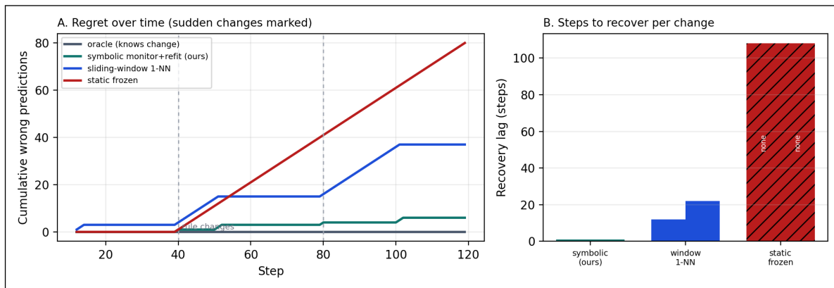
Figure 20: Adapting to sudden unannounced rule changes (E41). A reservoir’s hidden regime jumps at the marked steps; predictions run through the perception boundary. A: cumulative wrong predictions—the symbolic monitor (ours) stays nearly flat, the sliding-window learner steps up and slowly recovers, the static-frozen model climbs without bound, the oracle is flat at zero. B: recovery lag per change—1/1 steps for the symbolic monitor (to exact) versus 12/22 for the window; the frozen model never recovers.
