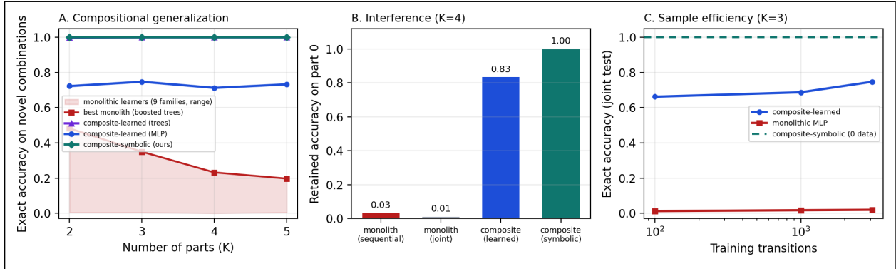
Figure 18: Composition vs. monolithic learners (E36) on a factored K -sector world, capacity-fair. A: exact accuracy on novel sector combinations—the whole monolithic family (shaded range over 9 learners; best, boosted trees, shown) collapses as K grows, while both composite learners and the symbolic composite stay flat near or at 1.0. B: accuracy retained on the first part after training through all K —the monolith suffers catastrophic interference, the composite does not. C: accuracy vs. training transitions—the composite learns from far less data, the symbolic composite from none.
