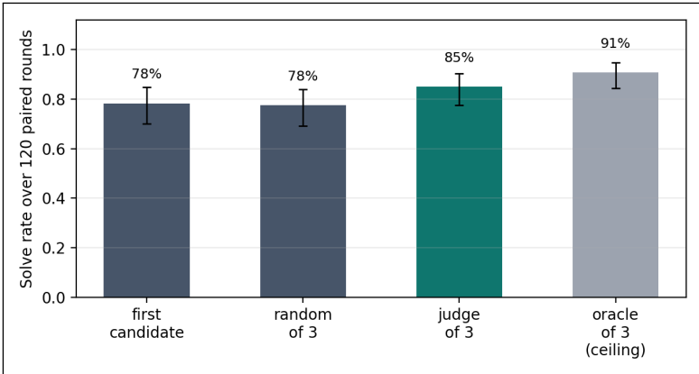
Figure 9: Controlled judge-selection comparison (E13+E17, pooled). Four selection strategies over the same three 1.5B candidate patches per round, 120 paired rounds; whiskers are 95% Wilson intervals. Random-of-3 isolates the diversity effect; the judge’s margin over it estimates the value of judgment (McNemar p = 0.078 , marginal).
