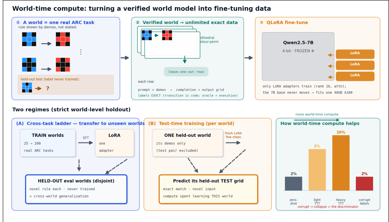
Figure 5: How world-time compute fine-tunes on a verified world model (E80, ARC-AGI).
