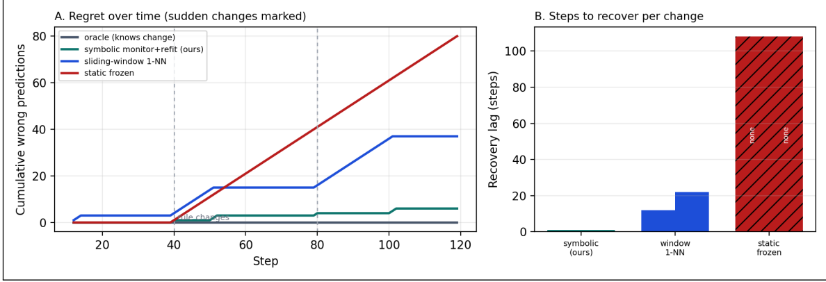
Figure 26: Adapting to sudden unannounced rule changes (E41). A reservoir’s hidden regime jumps at the marked steps; predictions run through the perception boundary. A: cumulative wrong predictions—the symbolic monitor (ours) stays nearly flat, the sliding-window learner steps up and slowly recovers, the static-frozen model climbs without bound, the oracle is flat at zero. B: recovery lag per change—1/1 steps for the symbolic monitor (to exact) versus 12/22 for the window; the frozen model never recovers.
