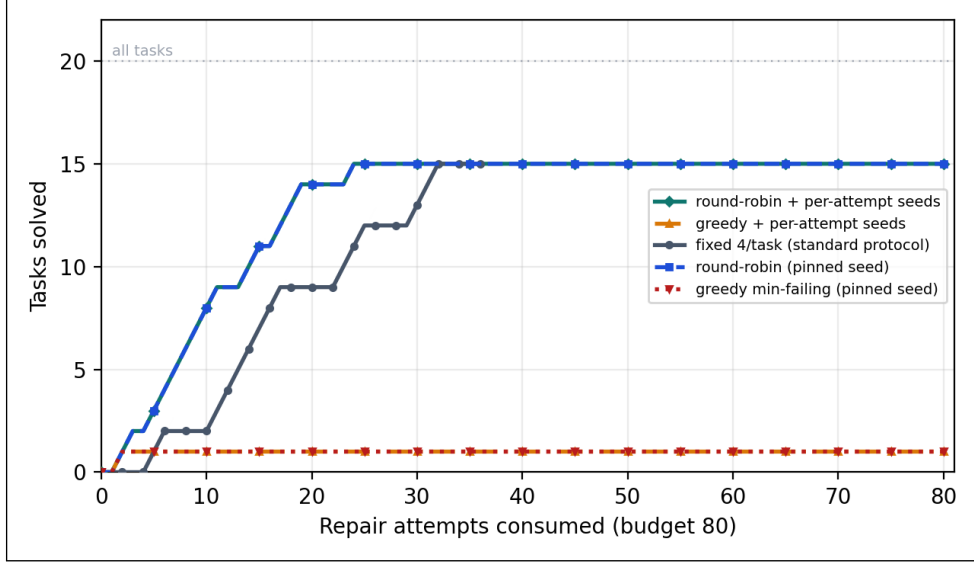
Figure 22: The sprint world (E34): tasks solved vs. repair attempts consumed on OpenWorld-SWE-bench (qwen2.5:7b, budget 80). The allocation policies act through the composite’s global view. No policy beats the fixed protocol’s ceiling—the unsolved tail is capability-bound, and greedy’s closest-to-passing heuristic tarpits on a single task with or without retry diversity—but round-robin reaches the plateau markedly faster.
