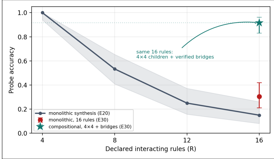
Figure 19: Composition defeats the cliff. The E20 curve (grey, with pooled 95% CI band): monolithic 7B synthesis accuracy falls as declared interacting rules grow. At R=16 , E30’s monolithic condition (red) lands on the fallen curve, while the same sixteen rules synthesized as four 4-rule children plus verified bridges (teal star) return to near- R=4 accuracy.
