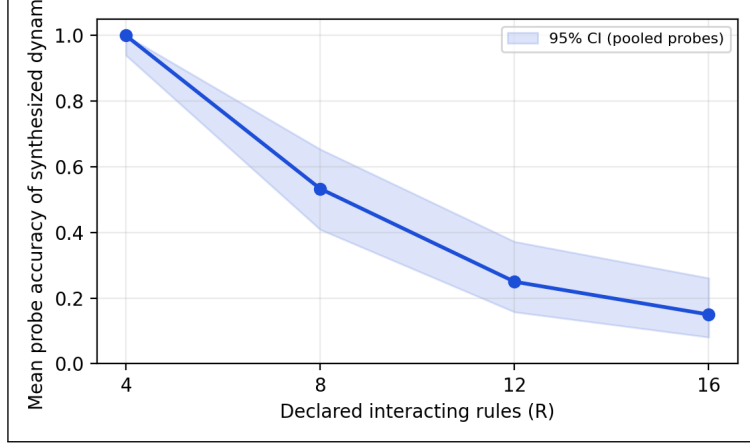
Figure 17: The complexity cliff (E20). Probe accuracy of 7B-synthesized dynamics versus the number of declared interacting rules; three syntheses per point, shaded band is the 95% CI over pooled probes. Monolithic synthesis is reliable at R=4 and unreliable past R\approx 8 .
