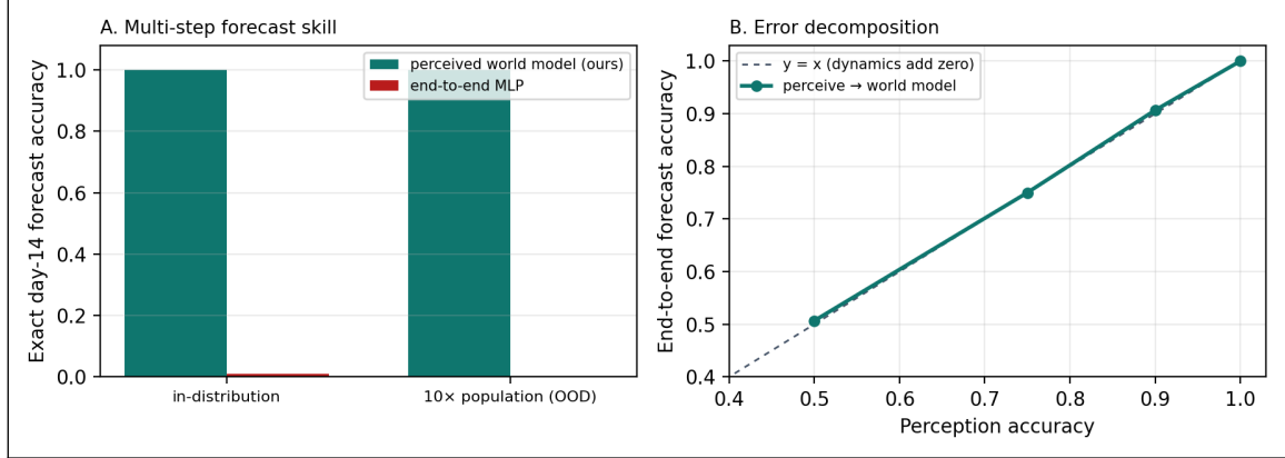
Figure 25: Perceive-then-forecast (E40). Multimodal day-0 inputs are perceived into the symbolic state of an SIR epidemic, then rolled forward 14 days by the verified world model. A: exact day-14 forecast accuracy—the perceived world model is exact in and out of distribution; the end-to-end MLP fails and collapses at 10\times scale. B: end-to-end forecast accuracy equals perception accuracy (the dynamics add zero error), so the system degrades only as fast as its perception does.
