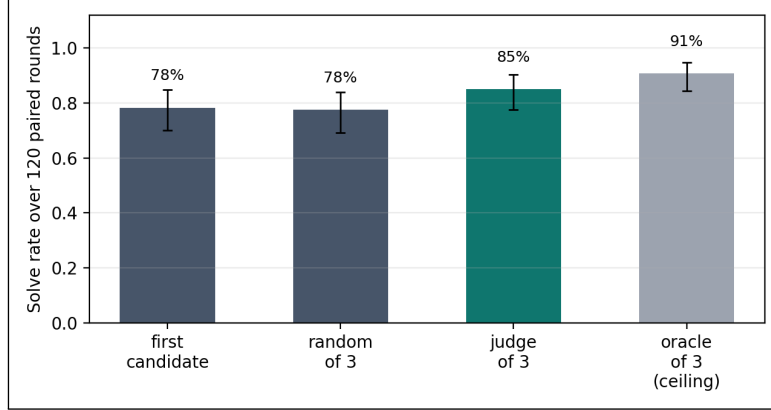
Figure 15: Controlled judge-selection comparison (E13+E17, pooled). Four selection strategies over the same three 1.5B candidate patches per round, 120 paired rounds; whiskers are 95% Wilson intervals. Random-of-3 isolates the diversity effect; the judge’s margin over it estimates the value of judgment (McNemar p = 0.078 , marginal).
