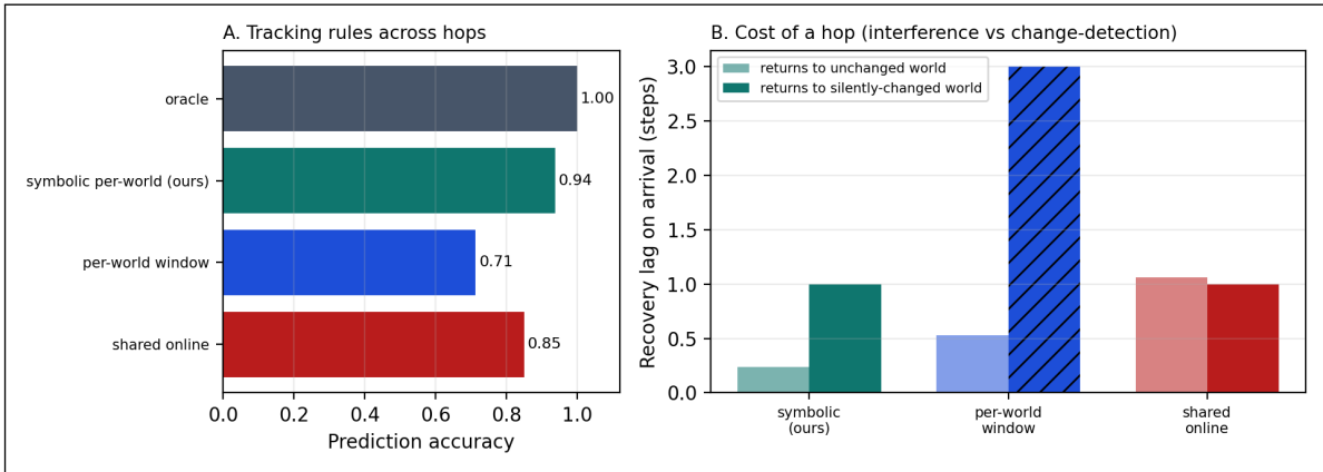
Figure 27: Agents traversing connected worlds with changing rules (E42). Two worlds joined by a toll route, each non-stationary, each with its own perception boundary; an agent hops between them. A: prediction accuracy tracking the current world’s rule across hops. B: recovery lag on arrival, split by whether the world’s rule changed while the agent was away. The shared-belief learner pays an interference cost even returning to an unchanged world; the per-world symbolic monitor returns nearly free and re-identifies away-changes in a step; the per-world window does not reliably recover from away-changes within a visit (hatched = no recovery).
