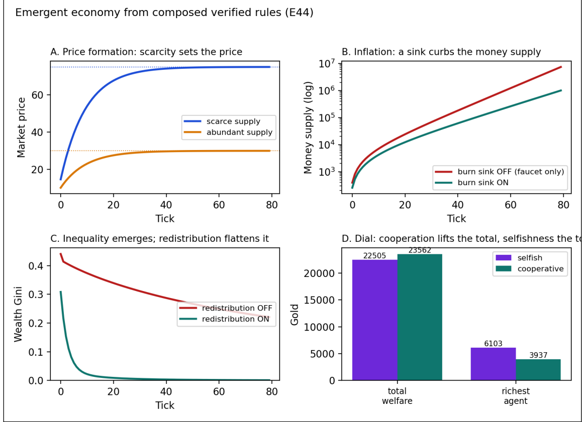
Figure 28: Emergent economy from composed verified rules (E44). Four macro phenomena, each isolated by toggling one verified rule. A: price converges to a supply-set level (scarcer supply \Rightarrow higher price). B: money supply (log) inflates with the burn sink off; the sink curbs it. C: the wealth Gini rises under selfish accumulation; redistribution flattens it. D: cooperation raises total welfare while selfishness produces the single richest agent. Nothing in the rules targets these quantities; they emerge and are causally attributed by separable toggles.
