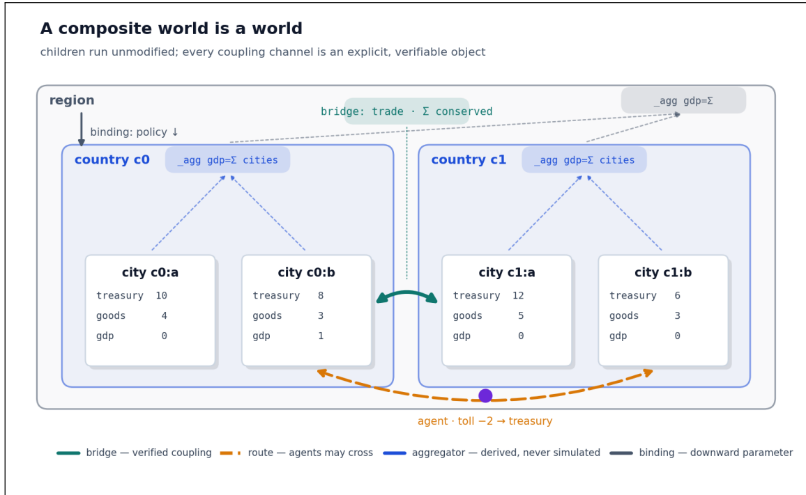
Figure 18: Anatomy of a composite world (the E31 system, real state values). Two country worlds, each containing two unmodified city worlds, compose into a region. The four coupling channels are explicit objects: a verified bridge carries trade under a conservation invariant; a dashed route lets an agent cross (paying a toll into the destination treasury); dashed upward arrows are aggregators —parent summaries derived from leaves, never independently simulated; the solid downward arrow is a binding injecting a parent parameter into a child.
