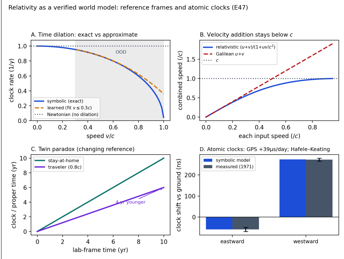
Figure 8: Relativity as a verified world model (E47). A: the moving-clock rate 1/\gamma —symbolic exact, a low-speed learned fit diverges OOD near c , Newtonian shows none. B: velocity addition stays below c ; the Galilean sum does not. C: the twin paradox as an agent worldline—the traveler returns 4 years younger. D: real atomic clocks—the model’s Hafele–Keating eastward/westward shifts vs. the 1971 measurements (GPS net +38.5 \mu\text{s/day} in the title).
