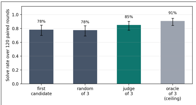
Figure 12: Controlled judge-selection comparison (E13+E17, pooled). Four selection strategies over the same three 1.5B candidate patches per round, 120 paired rounds; whiskers are 95% Wilson intervals. Random-of-3 isolates the diversity effect; the judge’s margin over it estimates the value of judgment (McNemar p = 0.078 , marginal).
