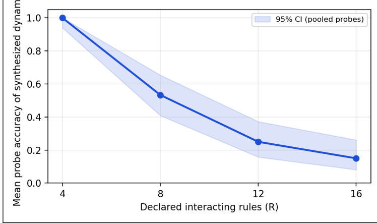
Figure 14: The complexity cliff (E20). Probe accuracy of 7B-synthesized dynamics versus the number of declared interacting rules; three syntheses per point, shaded band is the 95% CI over pooled probes. Monolithic synthesis is reliable at R=4 and unreliable past R\approx 8 .
