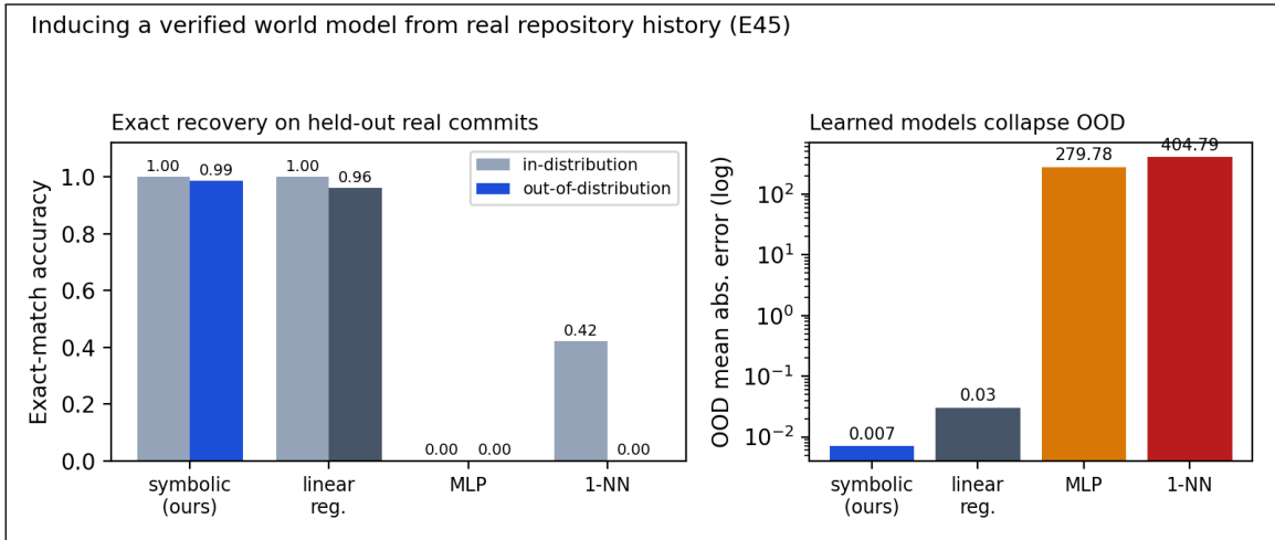
Figure 21: Inducing a verified world model from real repository history (E45). Mined from 3 real repos. Left: exact-match accuracy on held-out real commits, in-distribution and OOD (top-decile-churn commits). Only the symbolic program (and, for this linear law, linear regression) is exact; the neural MLP and the 1-NN memorizer are not. Right: OOD mean absolute error (log scale)—the learned world models miss by hundreds of lines, the induced program by a fraction of one.
