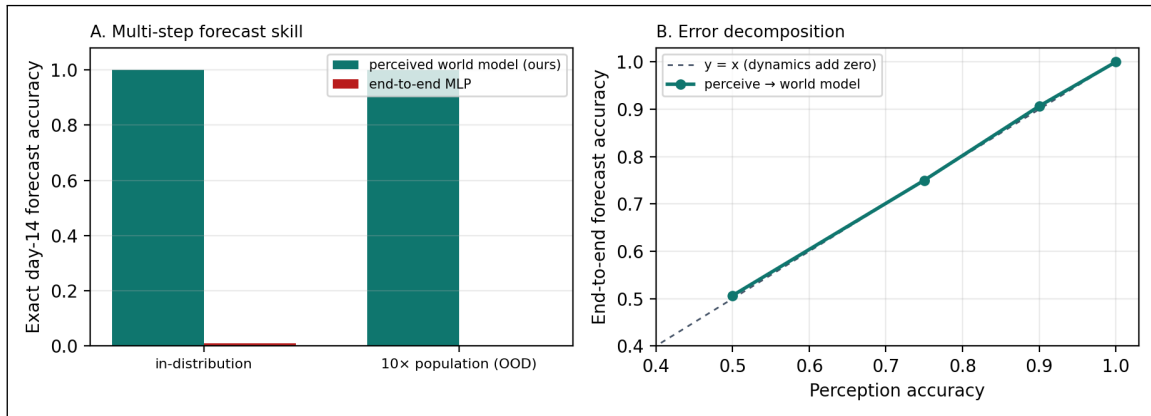
Figure 14: Perceive-then-forecast (E40). Multimodal day-0 inputs are perceived into the symbolic state of an SIR epidemic, then rolled forward 14 days by the verified world model. A: exact day-14 forecast accuracy—the perceived world model is exact in and out of distribution; the end-to-end MLP fails and collapses at 10 \times scale. B: end-to-end forecast accuracy equals perception accuracy (the dynamics add zero error), so the system degrades only as fast as its perception does.
