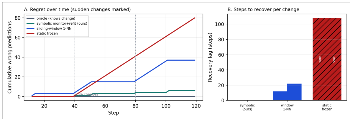
Figure 15: Adapting to sudden unannounced rule changes (E41). A reservoir’s hidden regime jumps at the marked steps; predictions run through the perception boundary. A: cumulative wrong predictions—the symbolic monitor (ours) stays nearly flat, the sliding-window learner steps up and slowly recovers, the static-frozen model climbs without bound, the oracle is flat at zero. B: recovery lag per change—1/1 steps for the symbolic monitor (to exact) versus 12/22 for the window; the frozen model never recovers.
