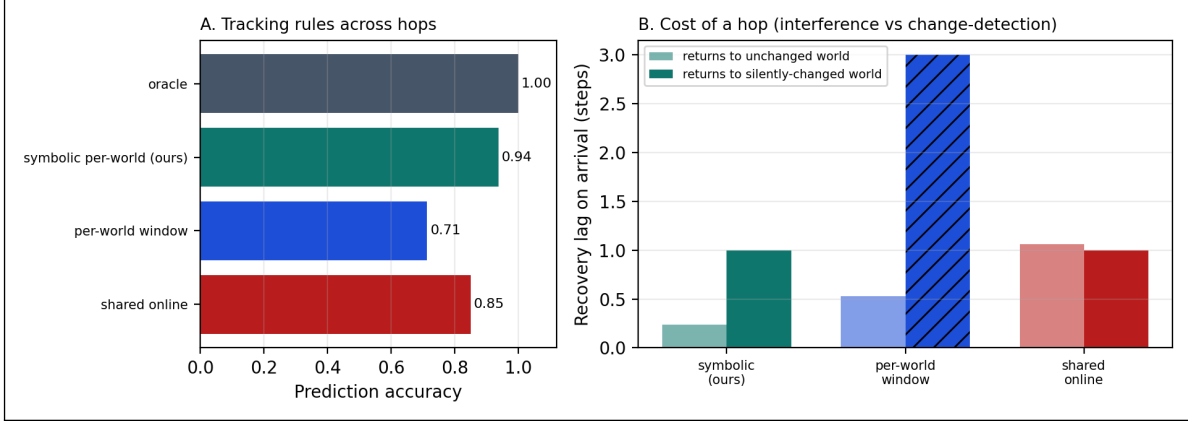
Figure 16: Agents traversing connected worlds with changing rules (E42). Two worlds joined by a toll route, each non-stationary, each with its own perception boundary; an agent hops between them. A: prediction accuracy tracking the current world’s rule across hops. B: recovery lag on arrival, split by whether the world’s rule changed while the agent was away. The shared-belief learner pays an interference cost even returning to an unchanged world; the per-world symbolic monitor returns nearly free and re-identifies away-changes in a step; the per-world window does not reliably recover from away-changes within a visit (hatched = no recovery).
