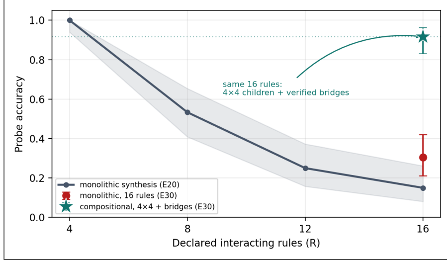
Figure 15: Composition defeats the cliff. The E20 curve (grey, with pooled 95% CI band): monolithic 7B synthesis accuracy falls as declared interacting rules grow. At R=16 , E30’s monolithic condition (red) lands on the fallen curve, while the same sixteen rules synthesized as four 4-rule children plus verified bridges (teal star) return to near- R=4 accuracy.
