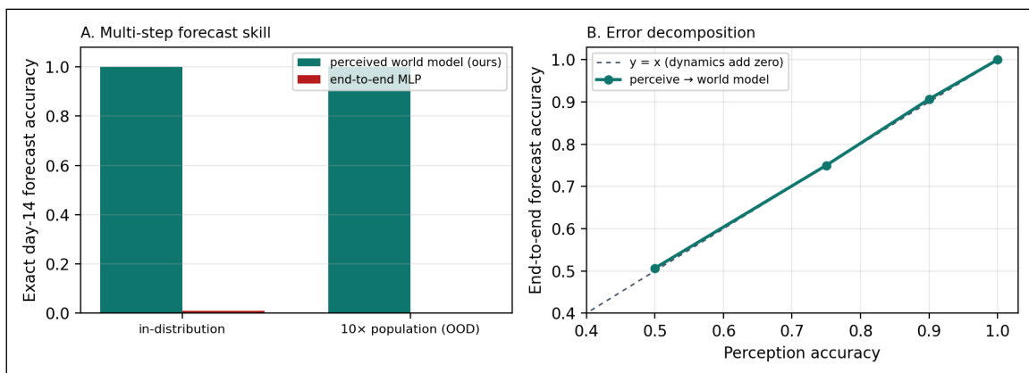
Figure 21: Perceive-then-forecast (E40). Multimodal day-0 inputs are perceived into the symbolic state of an SIR epidemic, then rolled forward 14 days by the verified world model. A: exact day-14 forecast accuracy—the perceived world model is exact in and out of distribution; the end-to-end MLP fails and collapses at 10\times scale. B: end-to-end forecast accuracy equals perception accuracy (the dynamics add zero error), so the system degrades only as fast as its perception does.
