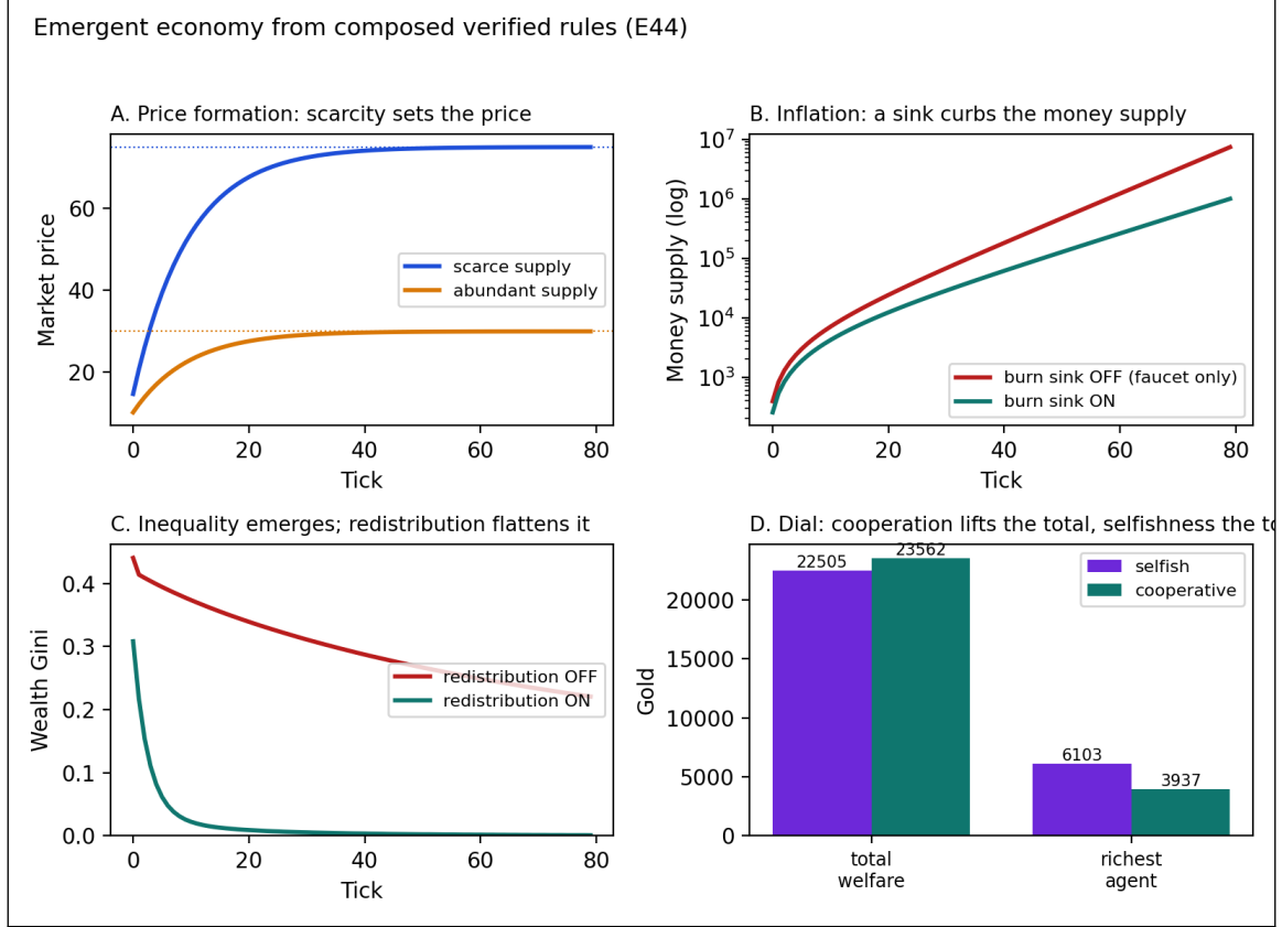
Figure 24: Emergent economy from composed verified rules (E44). Four macro phenomena, each isolated by toggling one verified rule. A: price converges to a supply-set level (scarcer supply \Rightarrow higher price). B: money supply (log) inflates with the burn sink off; the sink curbs it. C: the wealth Gini rises under selfish accumulation; redistribution flattens it. D: cooperation raises total welfare while selfishness produces the single richest agent. Nothing in the rules targets these quantities; they emerge and are causally attributed by separable toggles.
