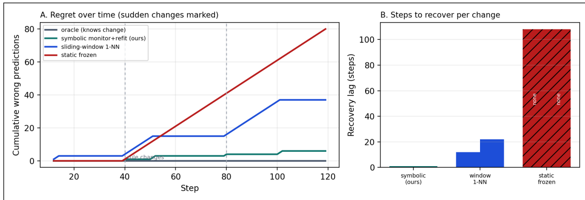
Figure 22: Adapting to sudden unannounced rule changes (E41). A reservoir’s hidden regime jumps at the marked steps; predictions run through the perception boundary. A: cumulative wrong predictions—the symbolic monitor (ours) stays nearly flat, the sliding-window learner steps up and slowly recovers, the static-frozen model climbs without bound, the oracle is flat at zero. B: recovery lag per change—1/1 steps for the symbolic monitor (to exact) versus 12/22 for the window; the frozen model never recovers.
