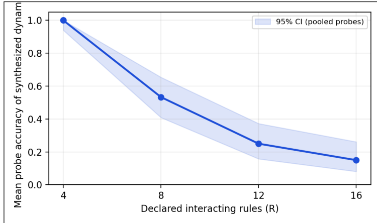
Figure 13: The complexity cliff (E20). Probe accuracy of 7B-synthesized dynamics versus the number of declared interacting rules; three syntheses per point, shaded band is the 95% CI over pooled probes. Monolithic synthesis is reliable at R=4 and unreliable past R \approx 8 .
