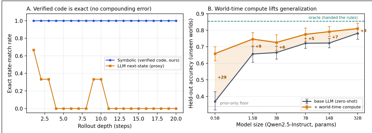
Figure 1: A : The task is to predict a world’s next symbolic state from the current state and an action (here the sprint backlog/debt/bug world, instrumented with a ground-truth oracle). Dynamics synthesized and verified once as code (blue) match the oracle exactly at every depth of a 20-step rollout, while per-step LLM next-state prediction (orange)—a structural stand-in for learned neural dynamics—first diverges at step 2.3 on average and never completes an exact rollout. (Panel A is the per-depth exact-match rate over n=3 rollouts—hence the orange trace is noisy and non-monotonic; the robust claim is the contrast with code’s exact-at-every-depth line, not the orange shape.) Programs encode rules, not statistics, so the compounding-error failure mode of learned world models is eliminated by construction, at zero training cost. B ( payoff ): what that exactness unlocks— world-time compute . Fine-tuning an LLM on trajectories traversed through 60 verified train world models lifts held-out diagnostic accuracy on 20 unseen worlds toward the rules-given oracle, with the largest gain for the smallest models (+29 points at 0.5B, shrinking to +3 at 32B)—a generalization lever that is strongest where capability is scarcest (bars: 95% bootstrap CIs over held-out specialties; dotted line: the prior-only floor; E74, §4.3).
