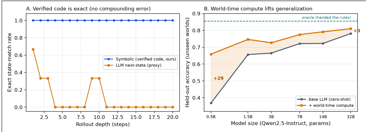
Figure 1: The paper in one figure. A (foundation) : On a ground-truth-instrumented world, dynamics synthesized and verified once as code (blue) match the oracle exactly at every depth of a 20-step rollout, while per-step LLM next-state prediction (orange)—a structural stand-in for learned neural dynamics—first diverges at step 2.3 on average and never completes an exact rollout. Programs encode rules, not statistics, so the compounding-error failure mode of learned world models is eliminated by construction, at zero training cost. B (payoff) : what that exactness unlocks— world-time compute . Fine-tuning an LLM on trajectories traversed through 60 verified train world models lifts held-out diagnostic accuracy on 20 unseen worlds toward the rules-given oracle, with the largest gain for the smallest models (+29 points at 0.5B, shrinking to +3 at 32B)—a generalization lever that is strongest where capability is scarcest (E74, §4.3).
