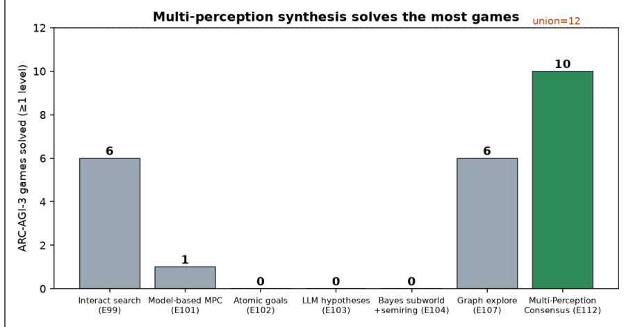
Figure 4: Games solved per strategy. Goal-discovery methods solve 0; directed search and graph exploration 6; multi-perception consensus solves 10 and adds four games no other method reaches (cn04, lf52, m0r0, s5i5). Across all strategies the union is 12/25.
