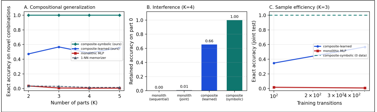
Figure 13: Composition vs. monolithic learners (E36) on a factored K -sector world, capacity-fair. A: exact accuracy on novel sector combinations—the composite is flat in K , the monolith and 1-NN collapse. B: accuracy retained on the first part after training through all K —the monolith suffers catastrophic interference, the composite does not. C: accuracy vs. training transitions—the composite learns from far less data, the symbolic composite from none.
