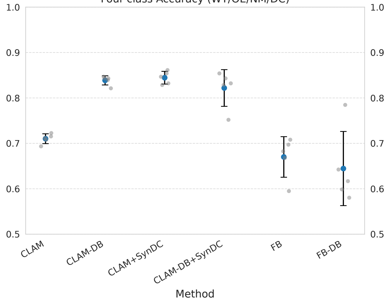
Four-class Accuracy (WT/OE/NM/DC)
