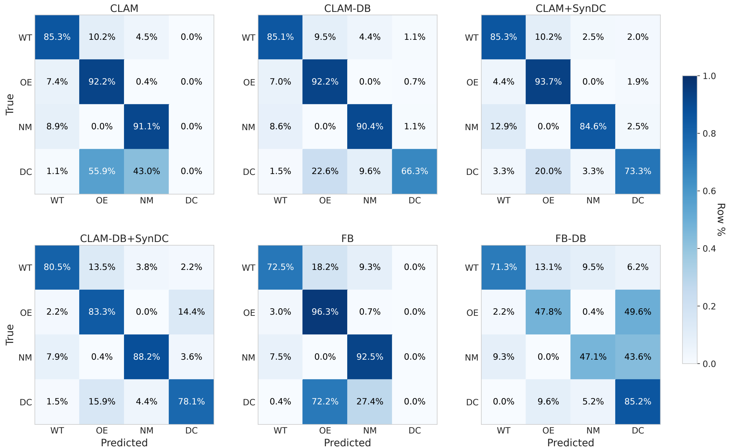
Confusion matrices per model
