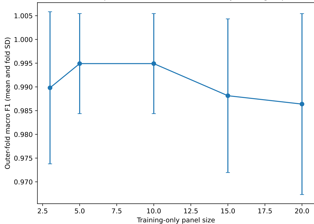
Task C tumor-normal panel size; final size chosen only within grouped inner CV
