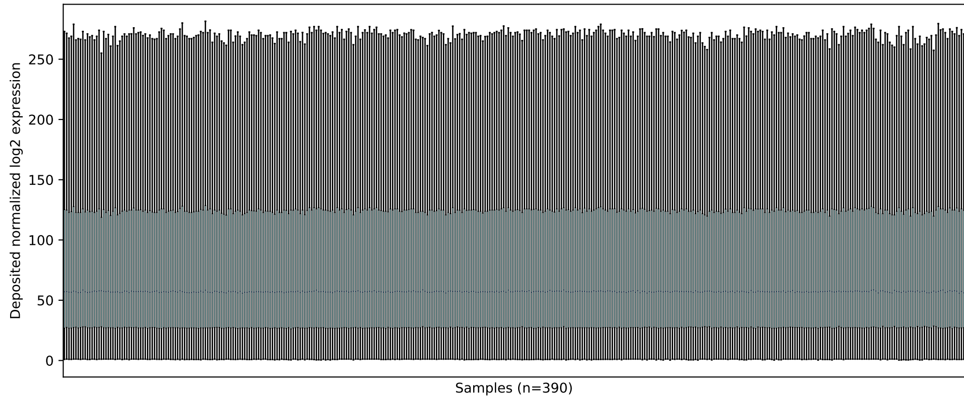
GSE41258: deposited normalized gene expression
