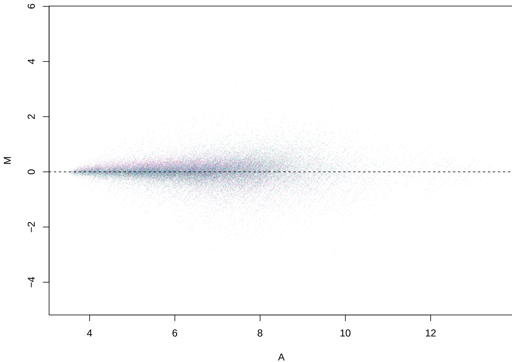
GSE41258 MA diagnostics (first six arrays)
