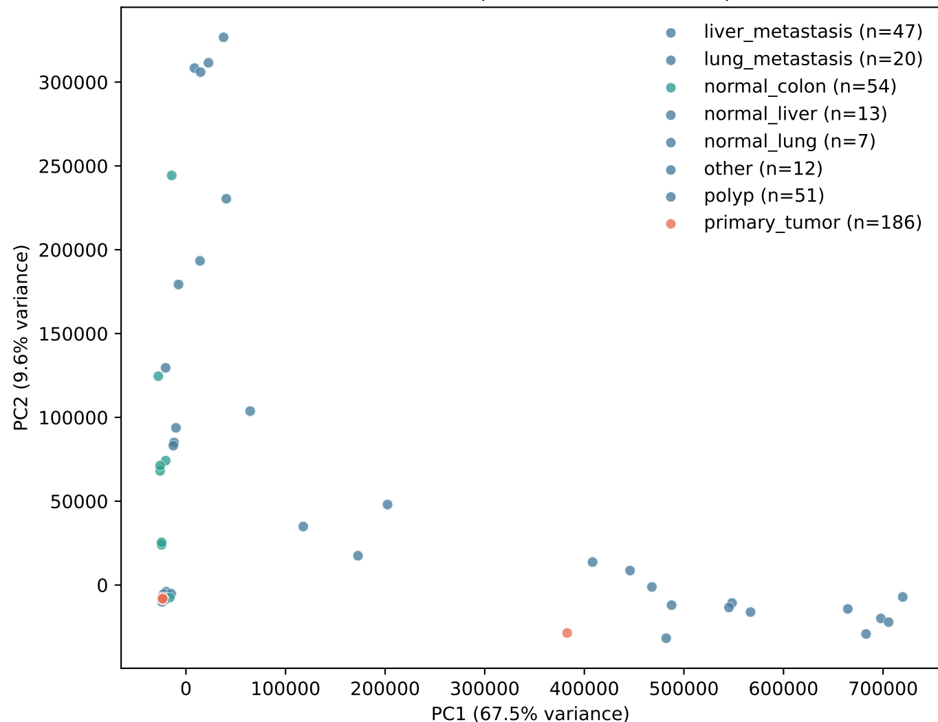
GSE41258: PCA of deposited normalized expression
